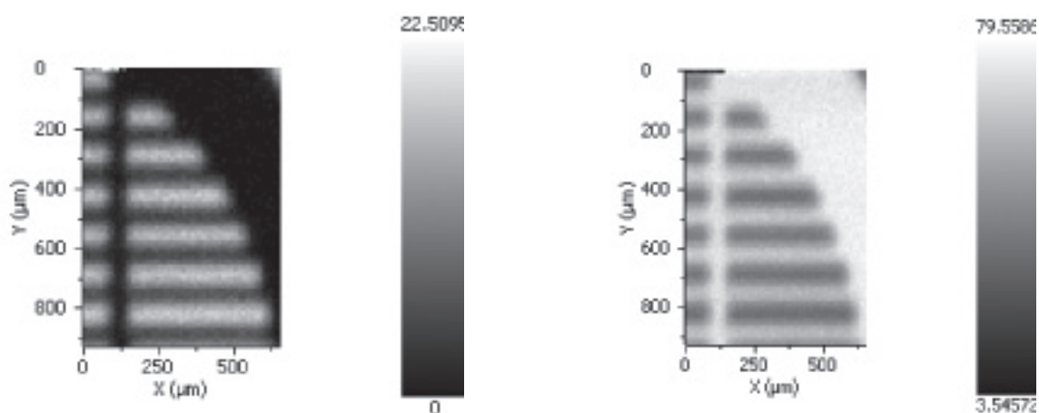
a) Atomic percent profile for C 1s CF 2
