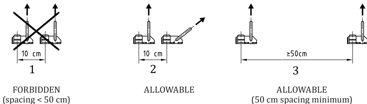
Figure 2 — Minimum distances
