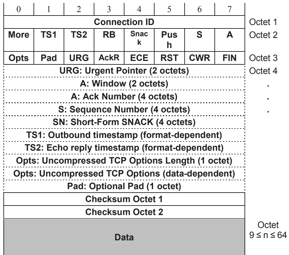
Figure 3-10: Compressed SCPS-TP Header
