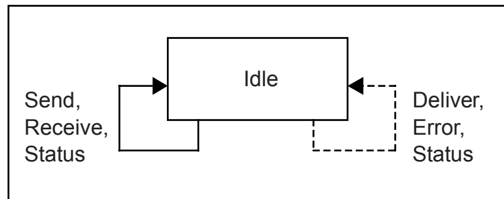
Figure D-4: State Diagram for Unacknowledged Service
