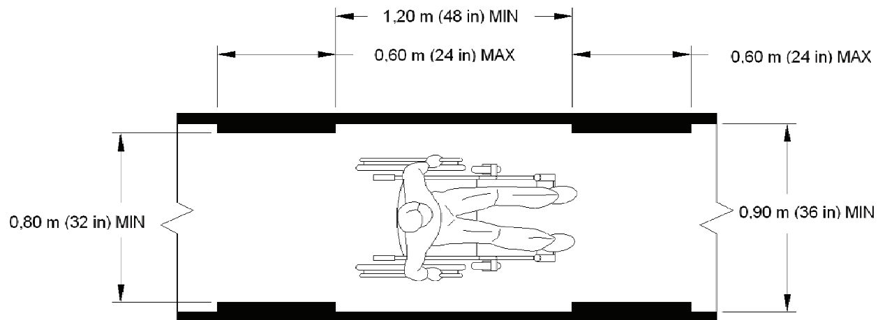
Figure A.2 — Clear pathway
