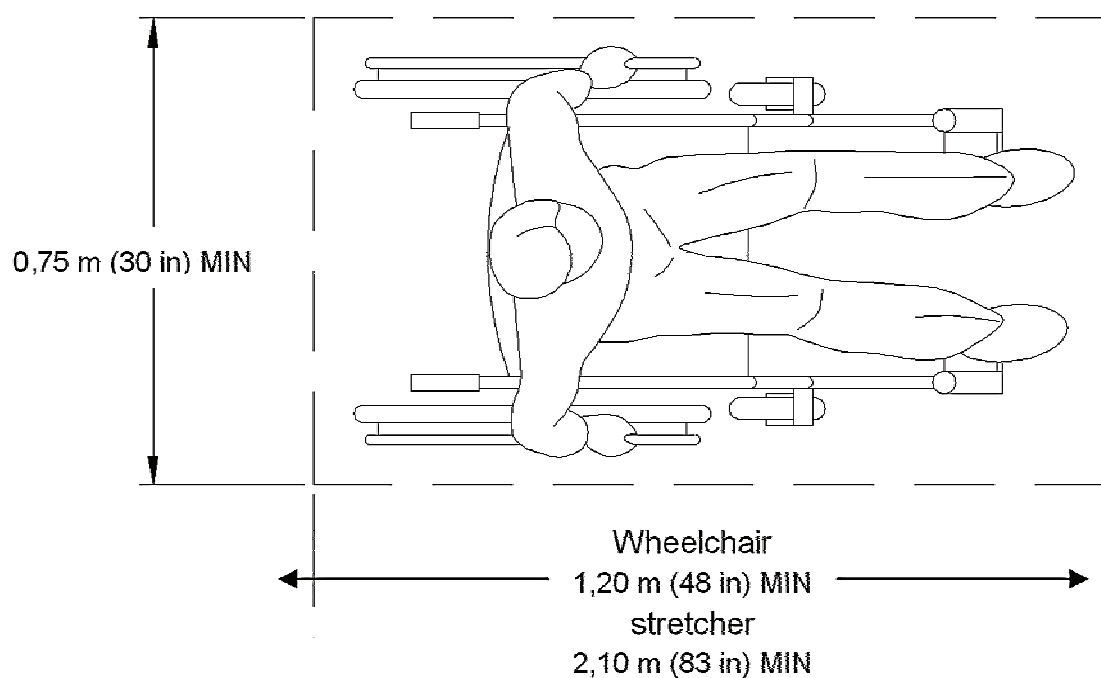
Figure A.1 — Clear floor space
