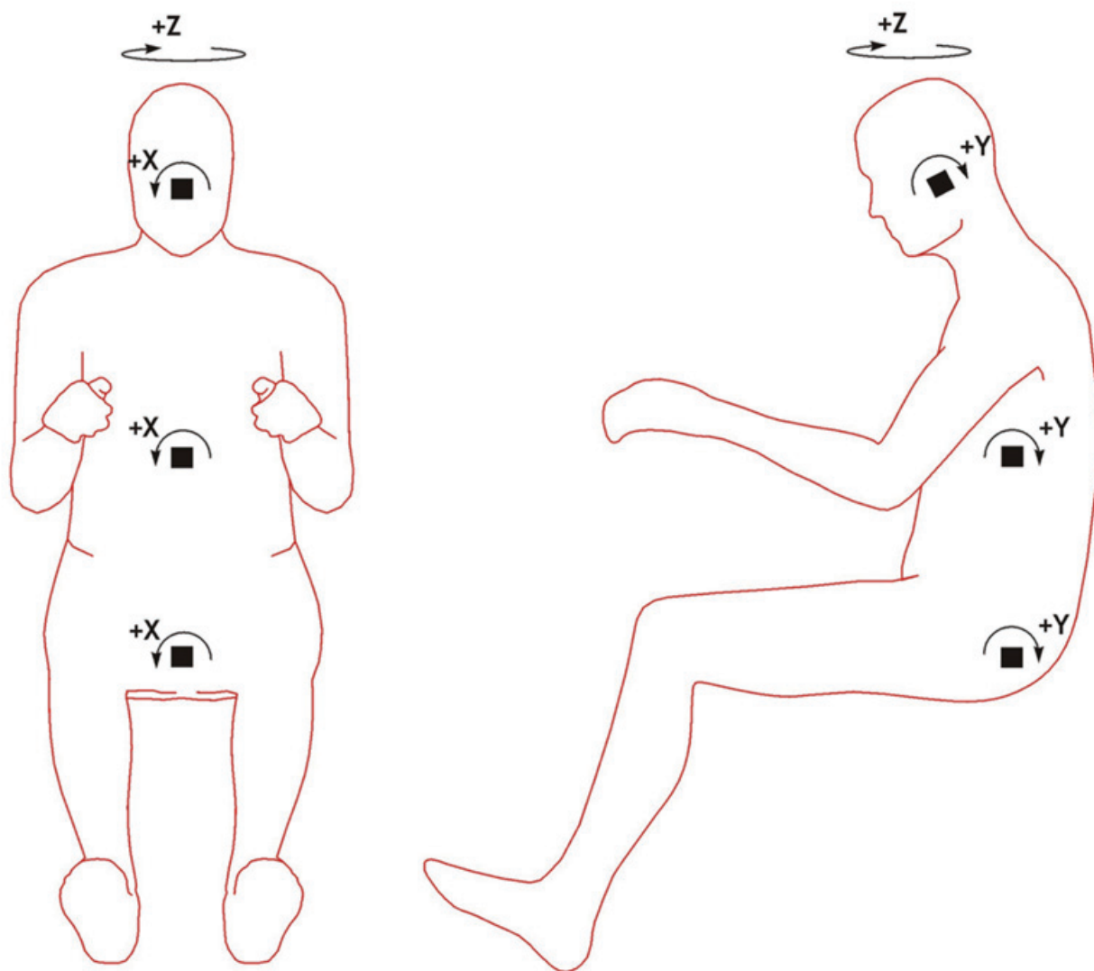
Figure D.17 — Tilt sensor channel orientations
