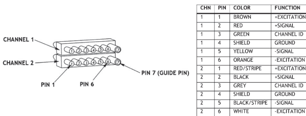
Figure B.7 — 2-channel connector to G5 DAS (configuration shown was only used in some WorldSID assemblies)
