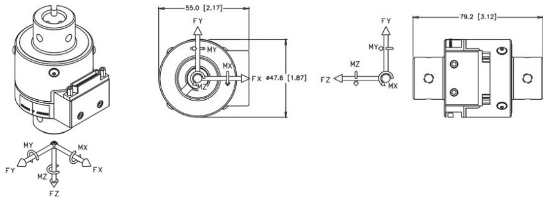
Figure A.6 — Femoral neck load cell
