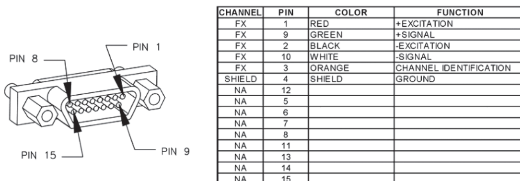
Figure B.5 — Connector wiring, 15-pin, 1 channel (side exit, pubic)
