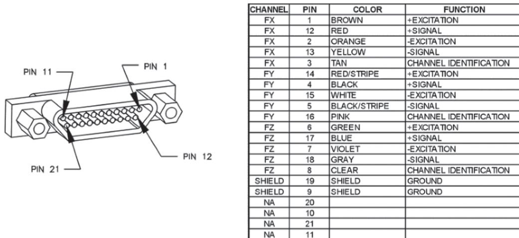
Figure B.3 — Connector wiring, 21-pin, 3 channels (shoulder)
