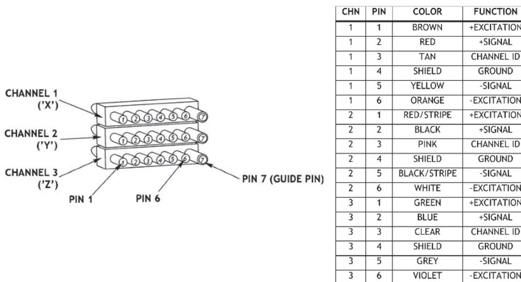
Figure B.8 — 3-channel connector to G5 DAS (configuration shown was only used in some WorldSID assemblies)
