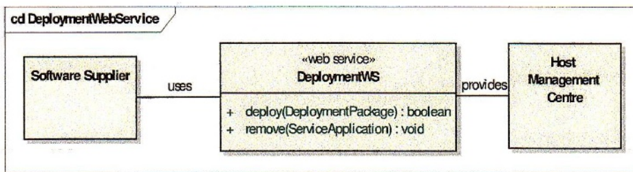
Figure B.2 — CVIS Figure 17 – Deployment API
