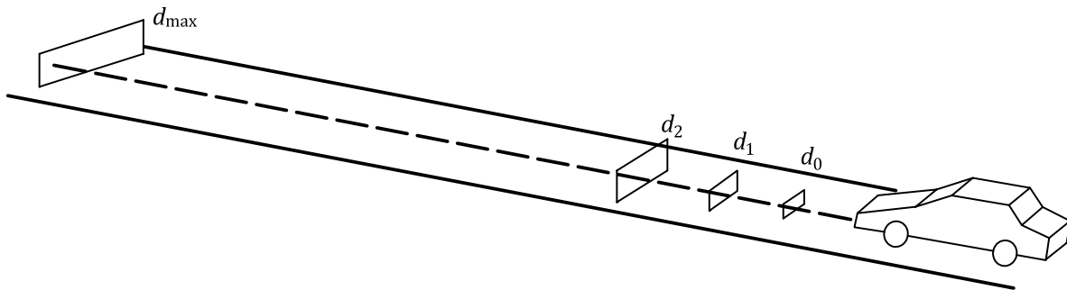
Figure 4 — Detection range
