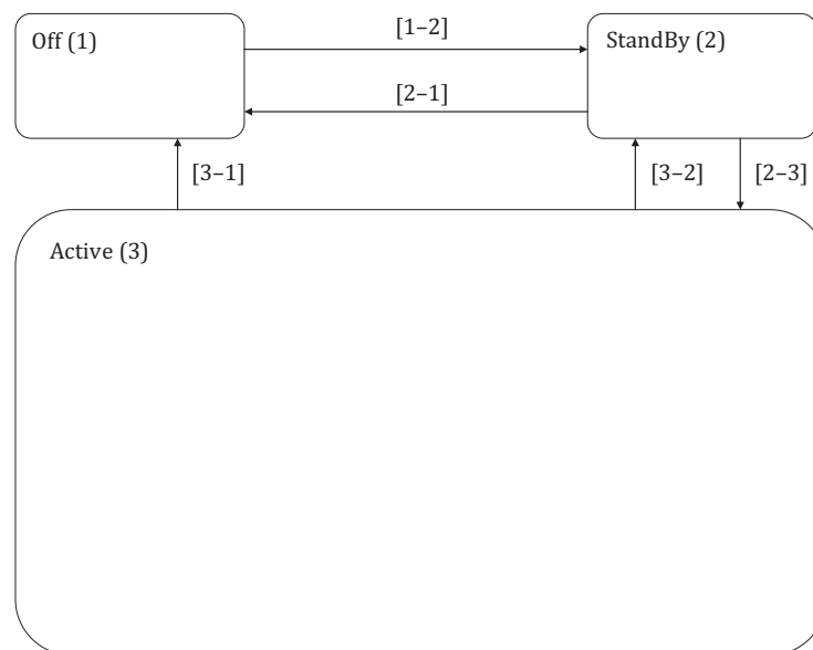
Figure 2 — FVCWS State Transition Diagram
