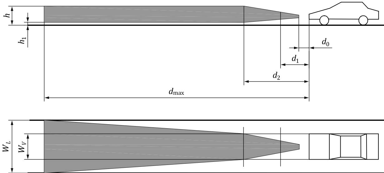
Figure 3 — Detection area
