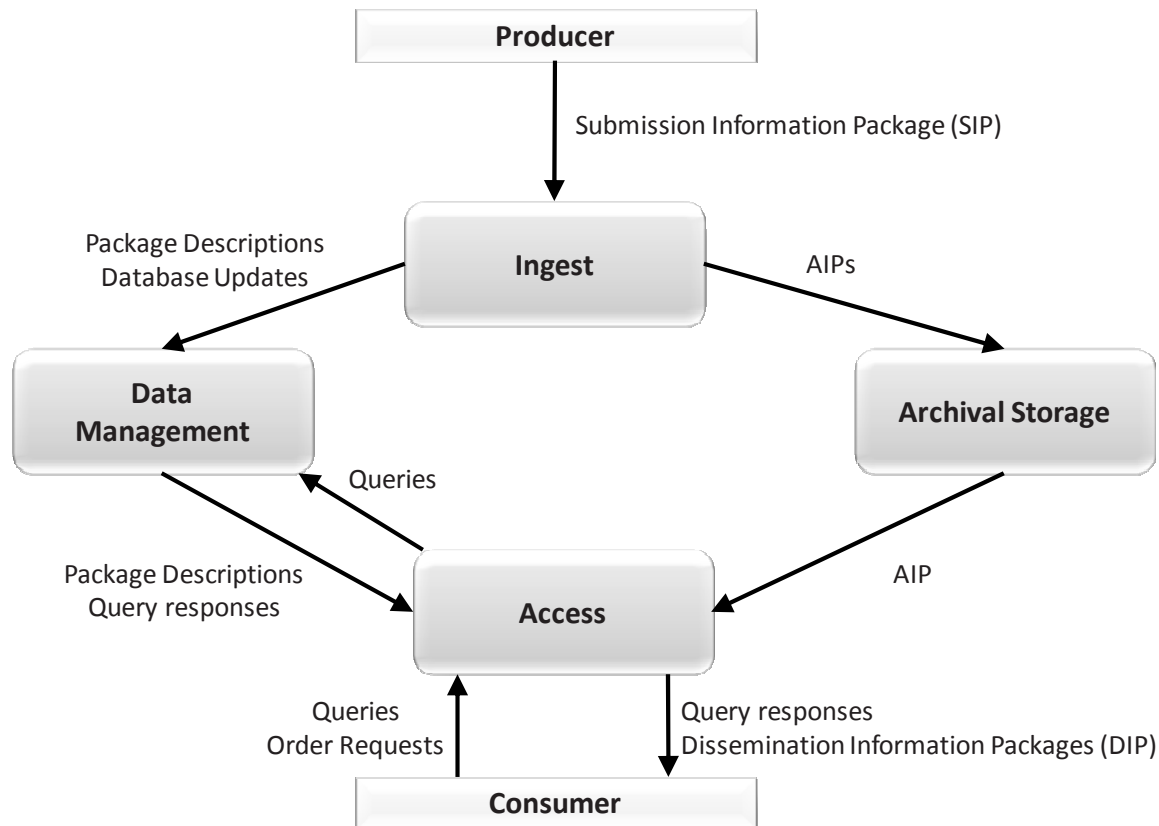
Figure 4-26: High-Level Data Flows in an OAIS
