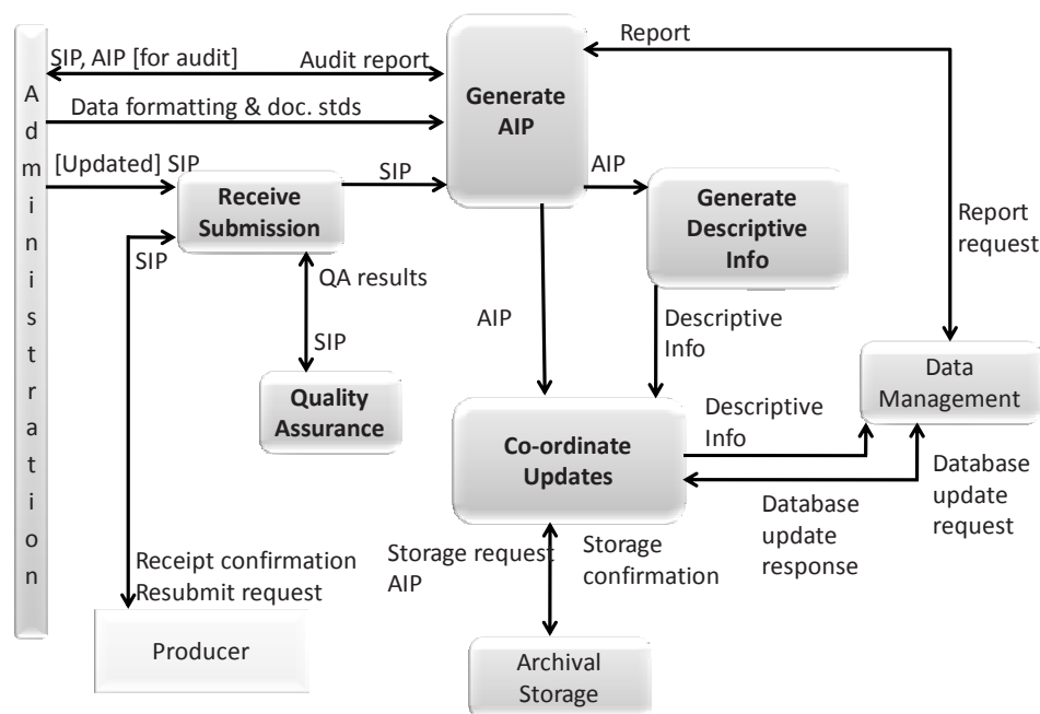
Figure 4-2: Functions of the Ingest Functional Entity
