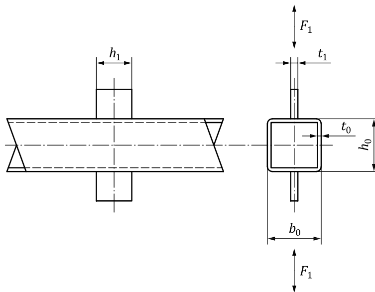
h) X-joint — longitudinal plate to RHS
