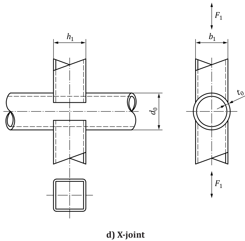
Figure 3 — Joints between open section or RHS braces and CHS chords
