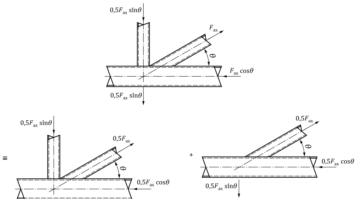
Figure 5 — Examples of hollow-section joint classification
