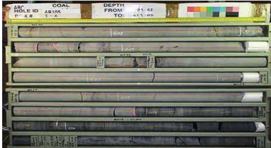
Figure 2 — Typical core box
