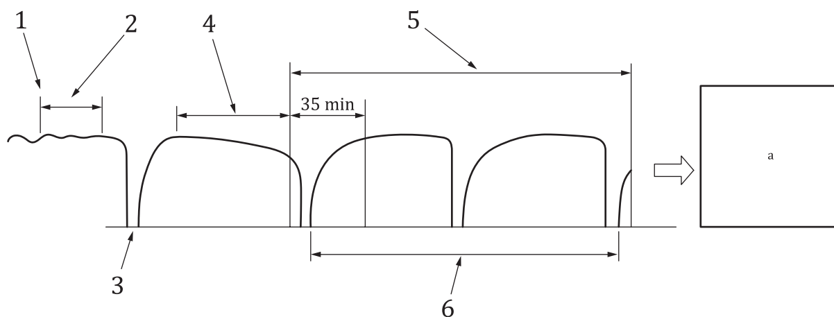
Figure M.5 — Transient heating capacity test with one complete cycle during the data collection period
