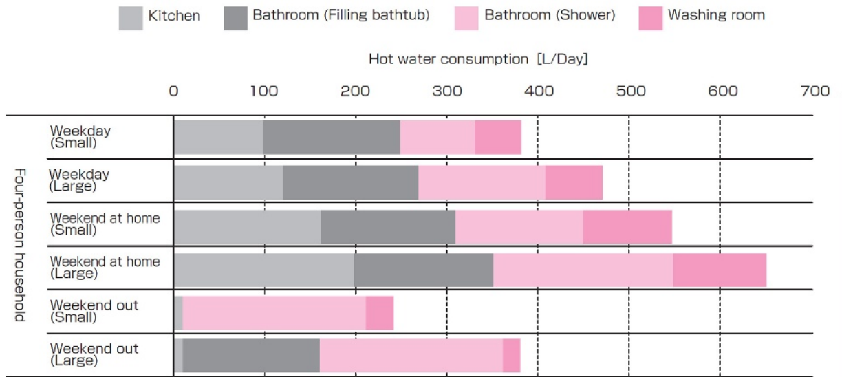
Figure A.4 — Hot water consumption during typical six days of “Corrected M1 Mode”
