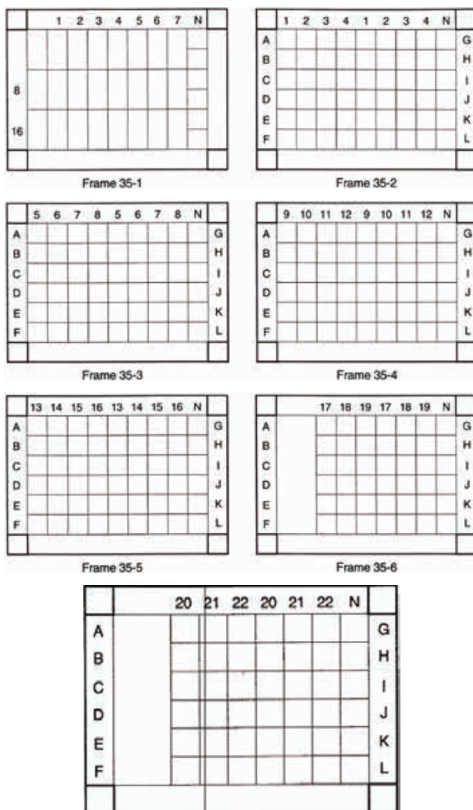
Figure 4 — Layout, Type 2 colour transmission target
