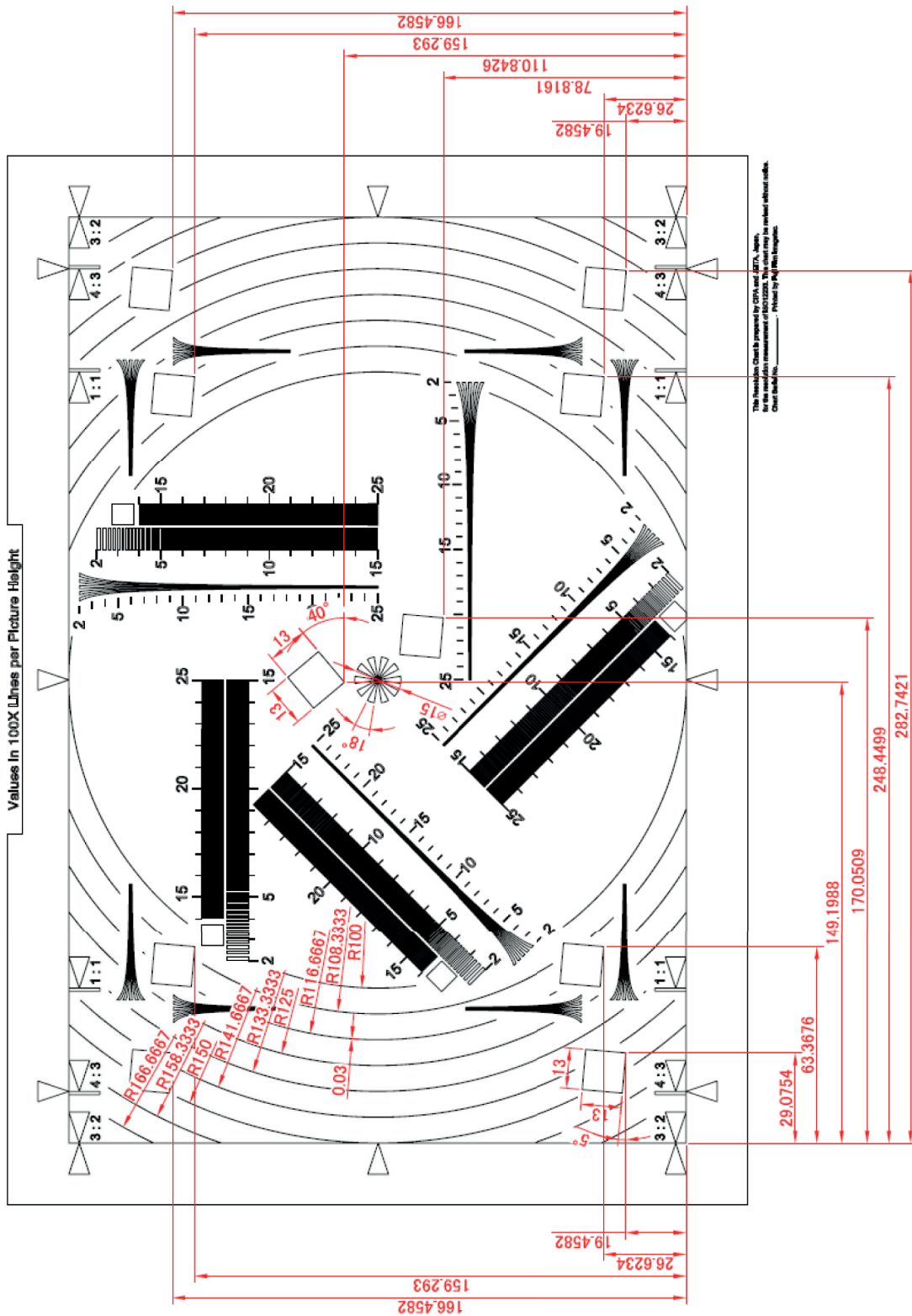
Figure A.3 — Dimensional drawing “B” for visual resolution target
