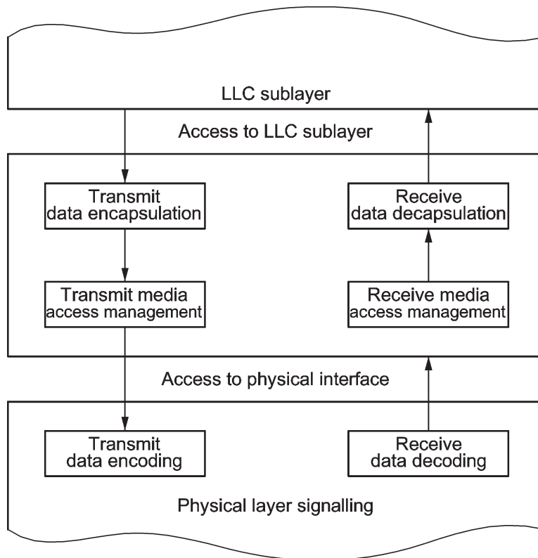
Figure 6 — MAC functions
