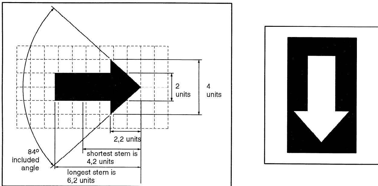
Figure D.24 — Arrow to represent exertion of pressure or force
