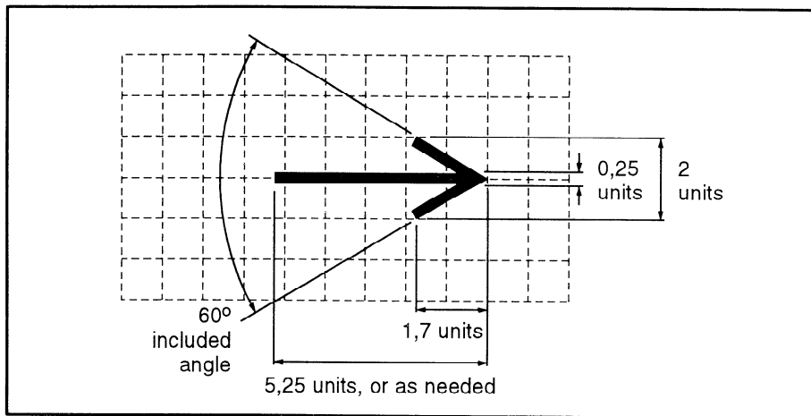
Figure D.20 — Arrow to represent direction of motion of machine components
