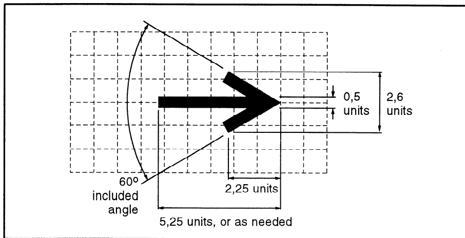
Figure D.22 — Arrow to represent direction of motion of entire machines
