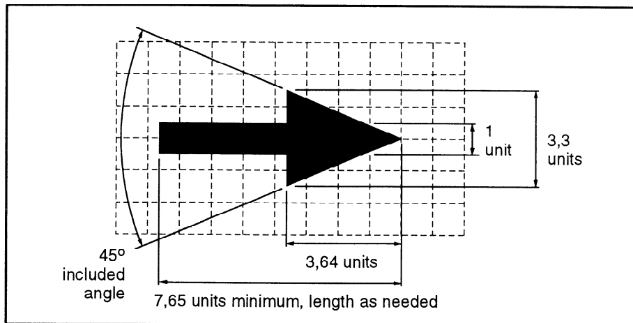
Figure D.18 — Arrow to represent falling or flying objects and their direction of motion
