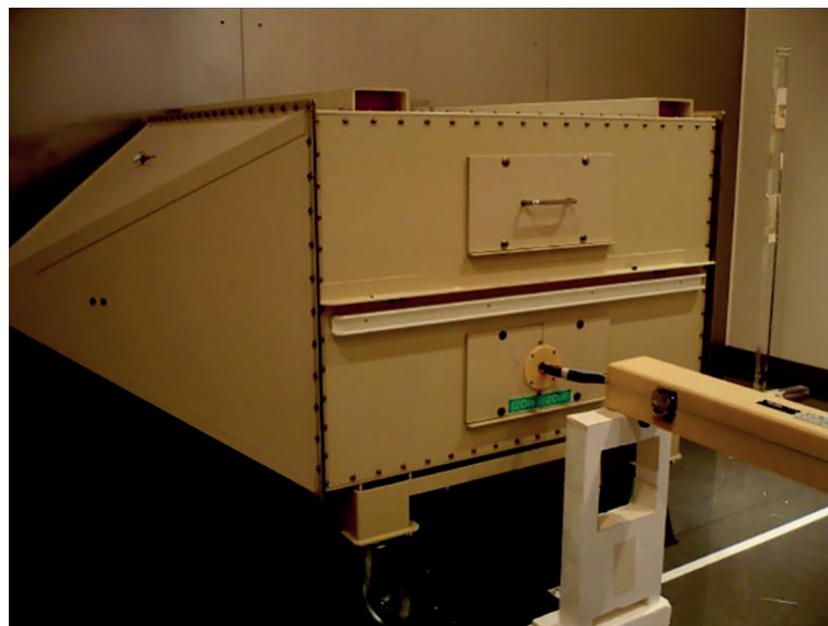
Figure D.5 — Example of test setup with a through-hole panel
