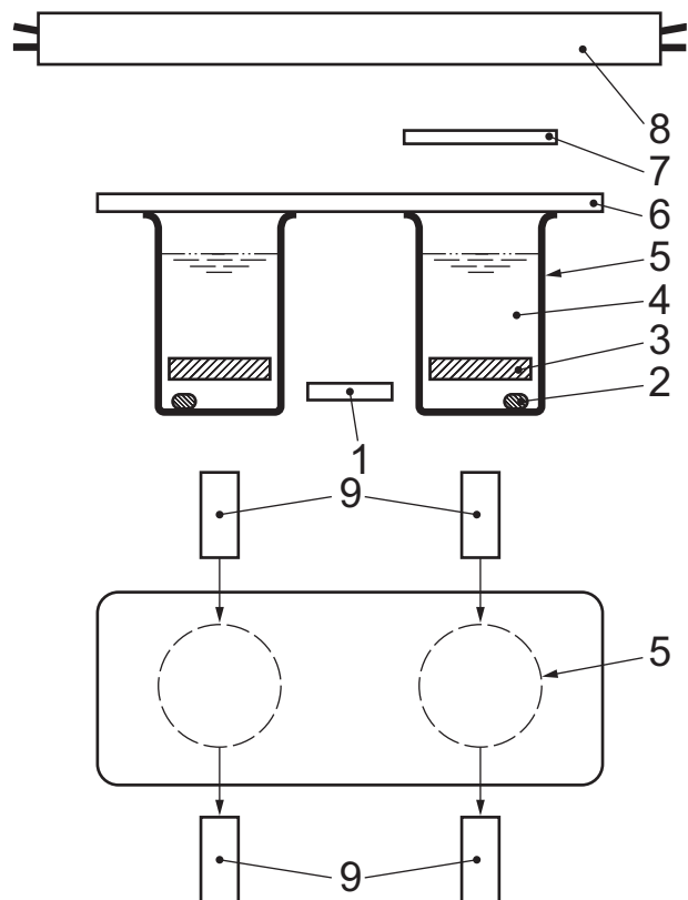
Figure B.2 — Schematic diagram of a measuring device with a testing cell
