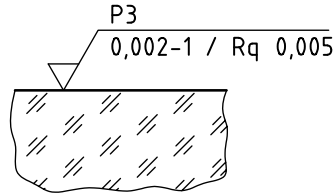
Figure 4 — Indication for optically smooth surface with quantitative modifiers; polishing grade of < 16 microdefects per 10 mm scan and R_q \leq 0,005 \mu\text{m} over a spatial bandwidth of 0,002 mm to 1 mm
