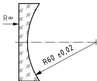
Figure 15 — Radii for a plano-concave lens element
