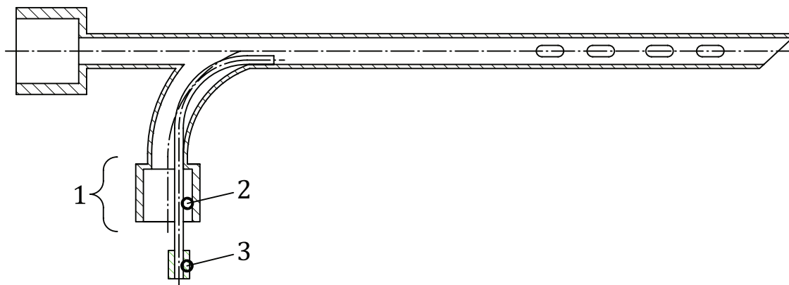
Figure 5 — Rigid bronchoscopes — Long jet-injector with specific lock
