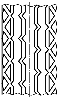
Figure A.1 — ISO SRTT — Tread pattern
