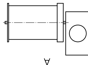
Single right-hand winch (R1)
