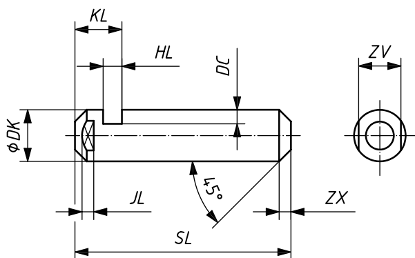
Figure 88 — AA6 - L: Pivot pin, spherical bearing, locking plate
