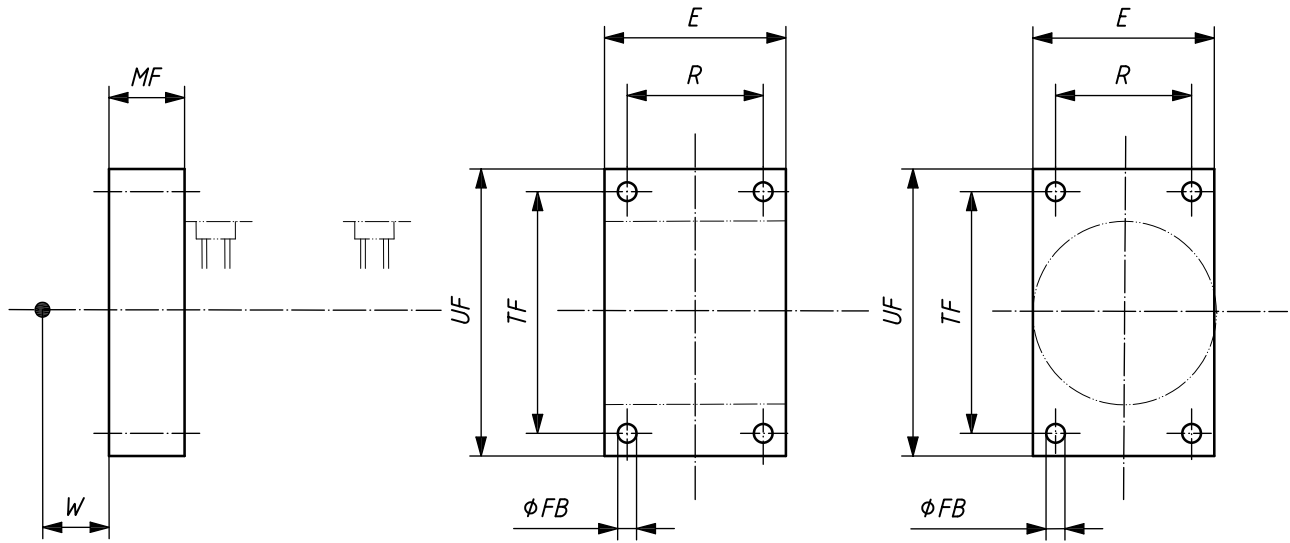
Figure 25 — MF 1: Head, rectangular flange
