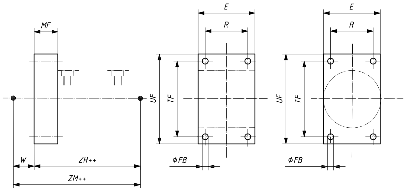
Figure 26 — MDF 1: Head, rectangular flange — Double rod
