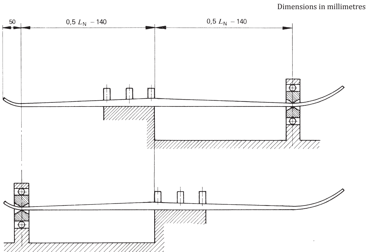
Figure 8 — Determination of forebody torsional spring constant, c_{TB} , and afterbody torsional spring constant, c_{TA}
