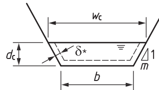
b) Section in approach channel upstream from throat
