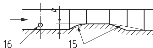
c) Longitudinal section of flume with raised invert (hump)
