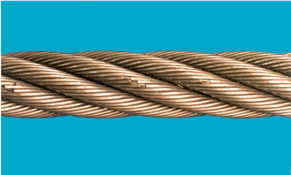
Figure B.13 — Crown wire breaks
