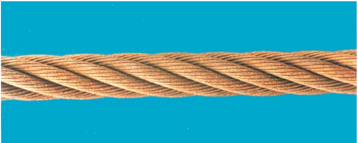
Figure B.11 — External corrosion
