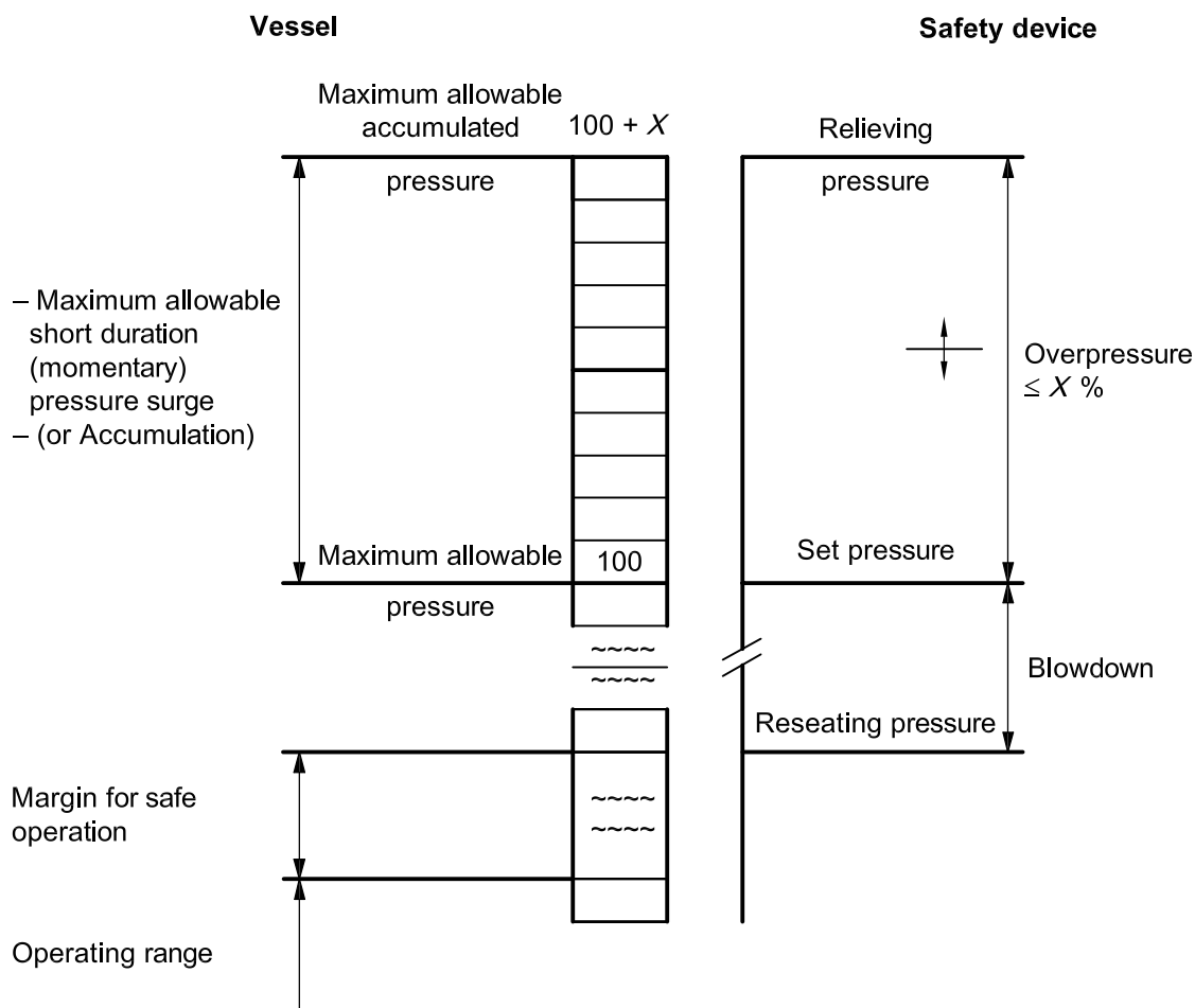
Figure A.1 — Safety valve applications — Safety valve certified at X % overpressure or less
