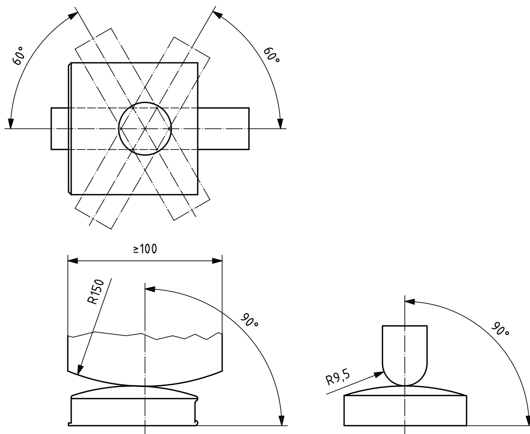
Figure 4 — Buckle compression
