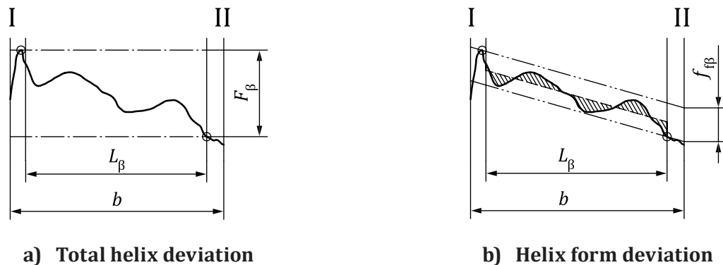
Figure 15 — Helix excess
