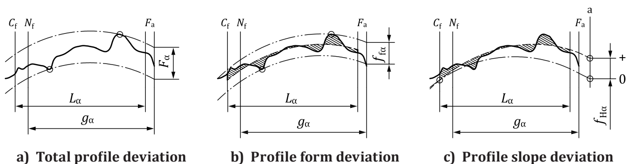
Figure 5 — Profile deviations with pressure angle modified
