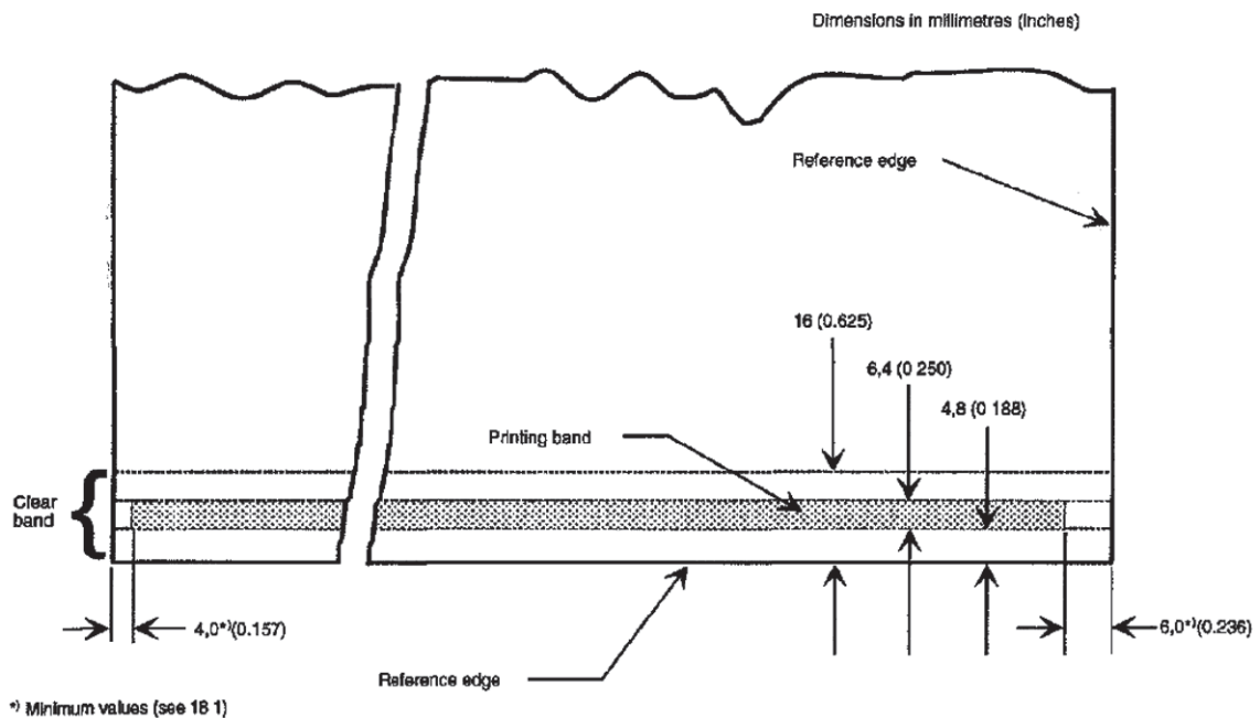
Figure 1 — Format of documents
