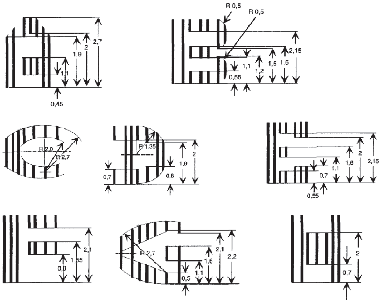
Figure 20 — Letter A to H: Font height 2,70 mm ( H_{14} )
