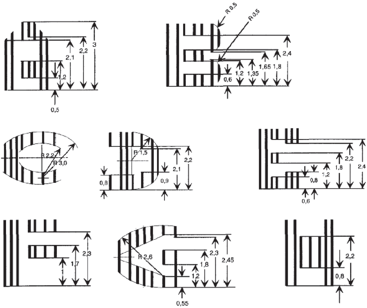
Figure 10 — Letters A to H: Font height 3,00 mm ( H_{12} )
