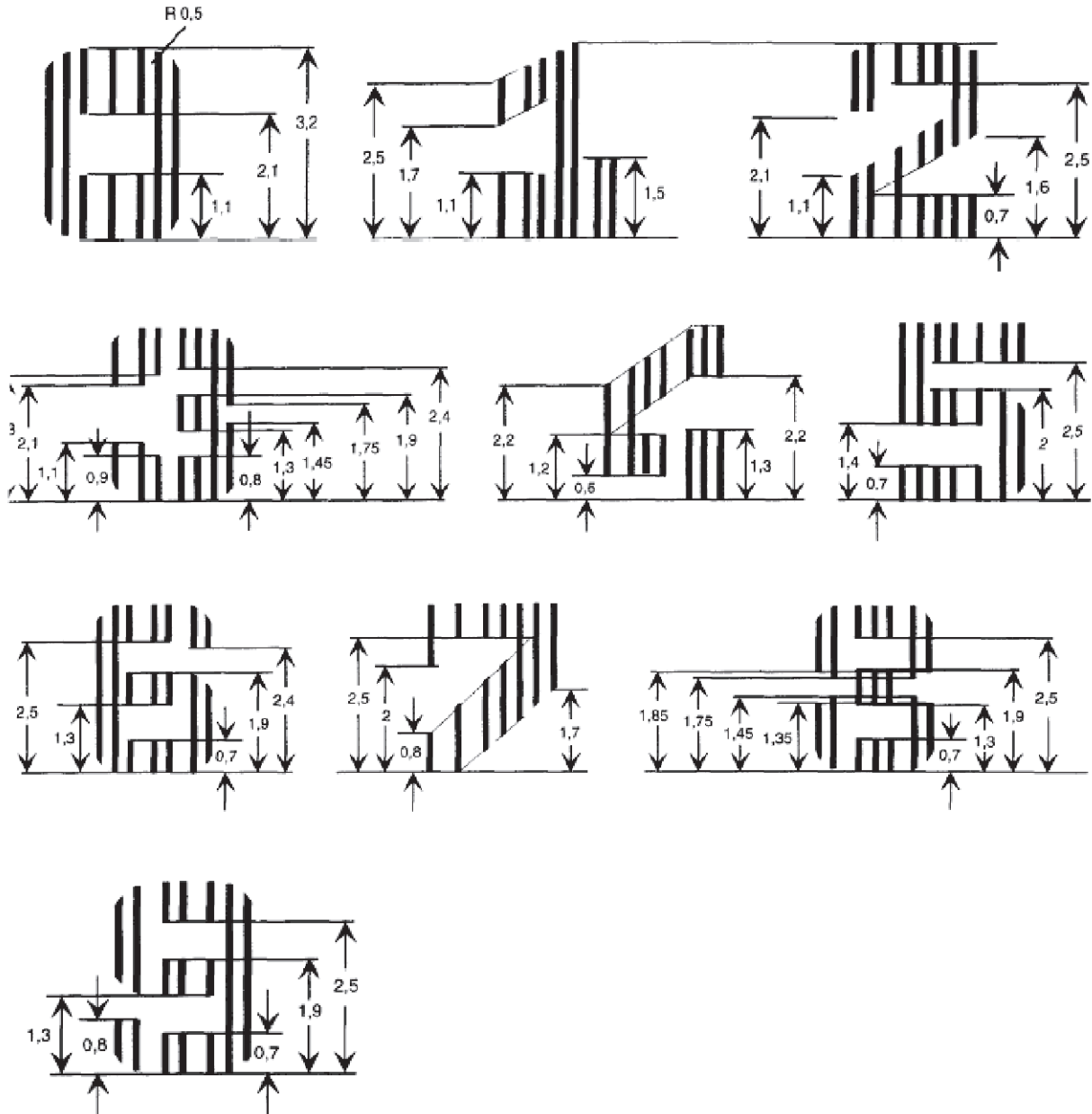
Figure 3 — Digits: Font height 3,20 mm ( H_{11} )
