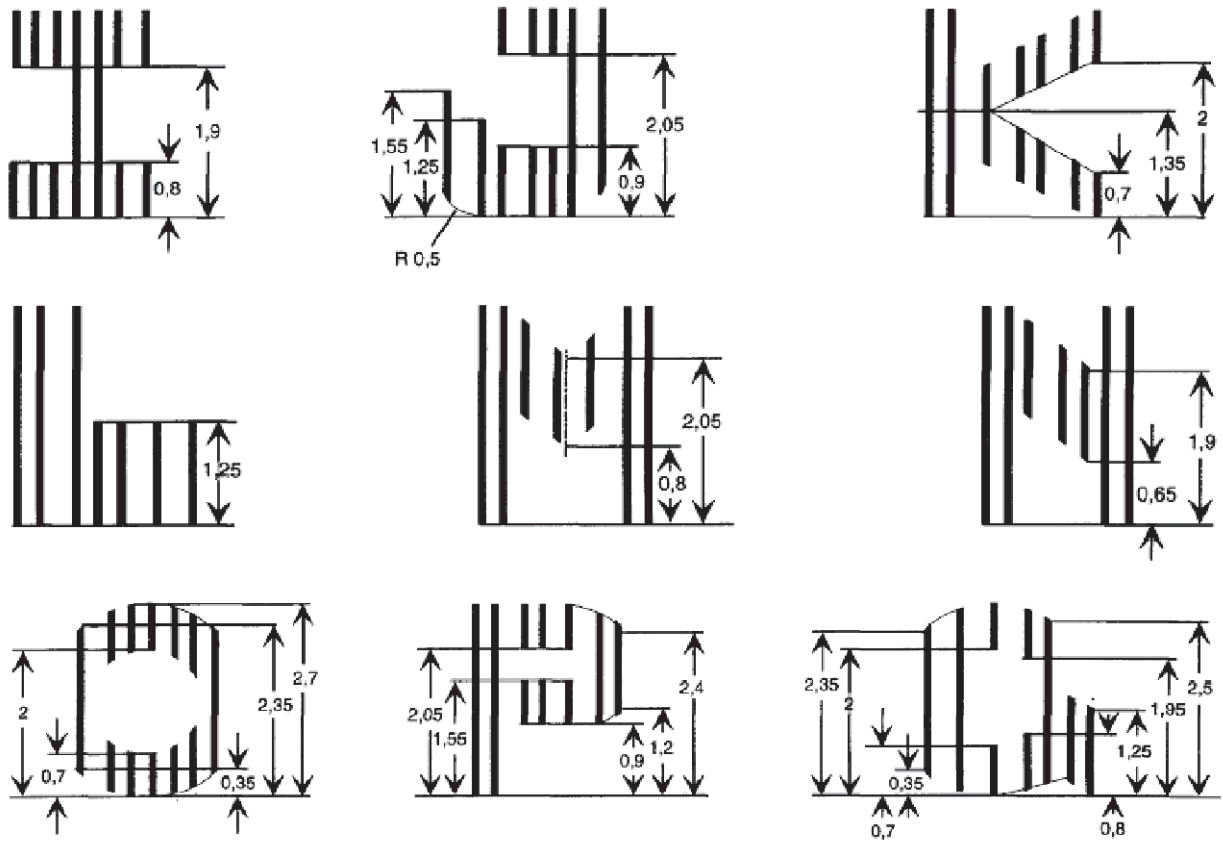
Figure 21 — Letter I to Q: Font height 2,70 mm ( H_{14} )
