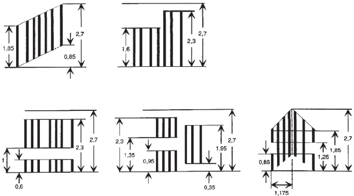
Figure 19 — Symbols: Font height 2,70 mm ( H_{14} ) (top row, left to right: S I, S II; bottom row, left to right: S III, S IV, S V)
