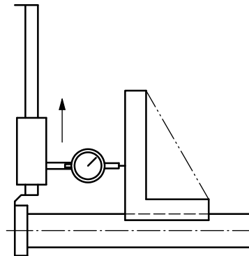
Figure 143 — Measurement of squareness error between an axis of linear motion and a stationary axis
