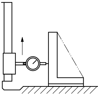
Figure 142 — Measurement of squareness error between an axis of linear motion and a plane
