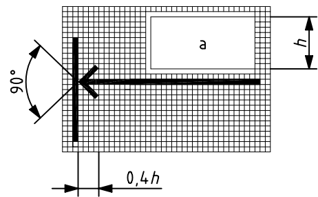
d) Arrowhead, open, included angle 90°
