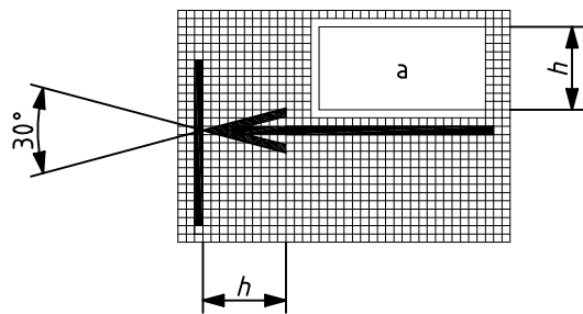
c) Arrowhead, open
