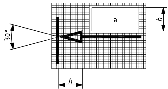
b) Arrowhead, closed
