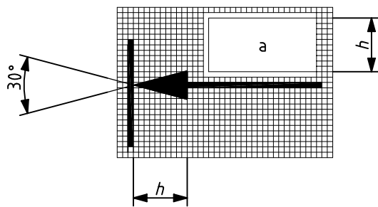
a) Arrowhead, closed and filled
