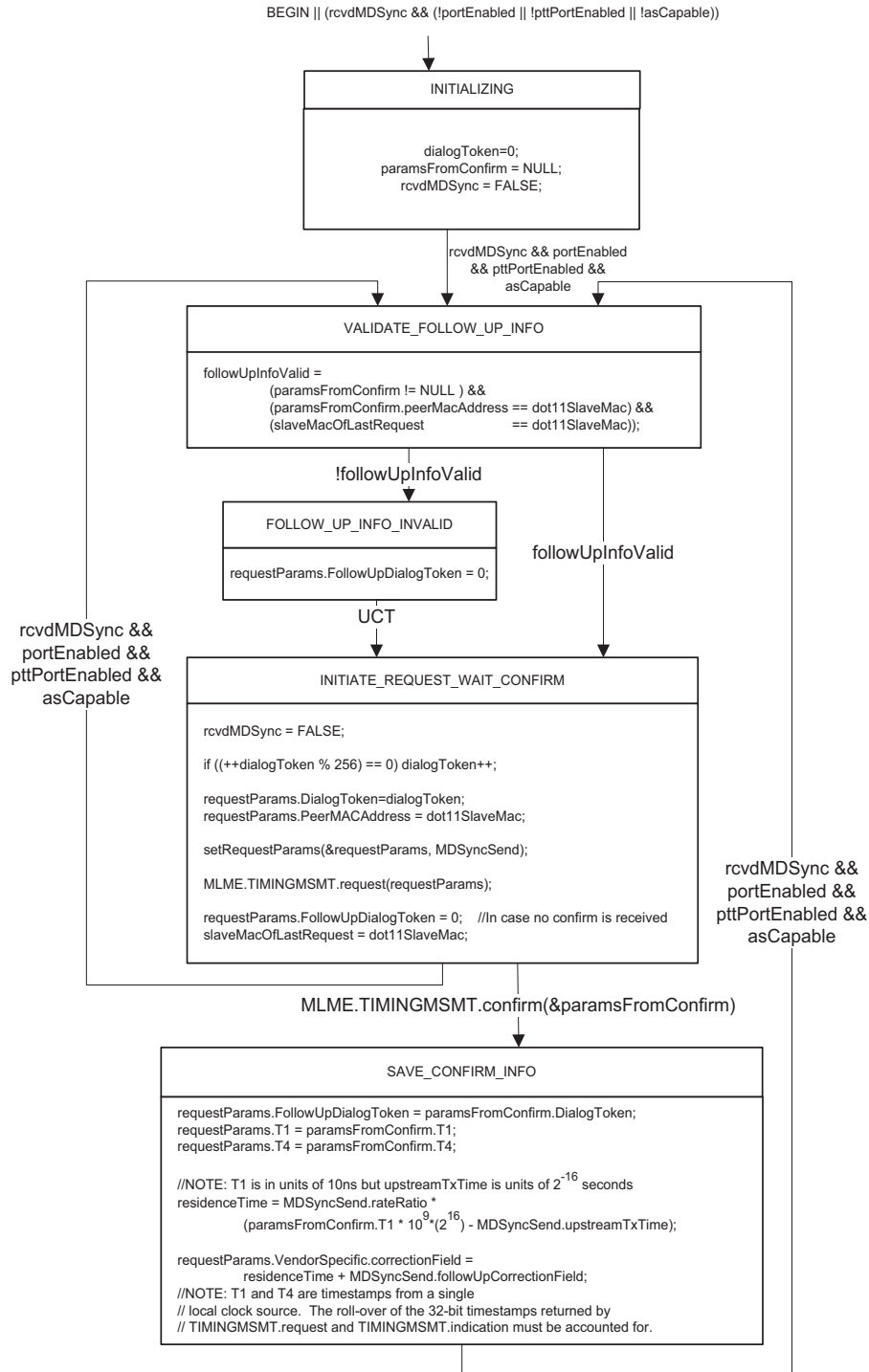
Figure 12-3—Master state machine
