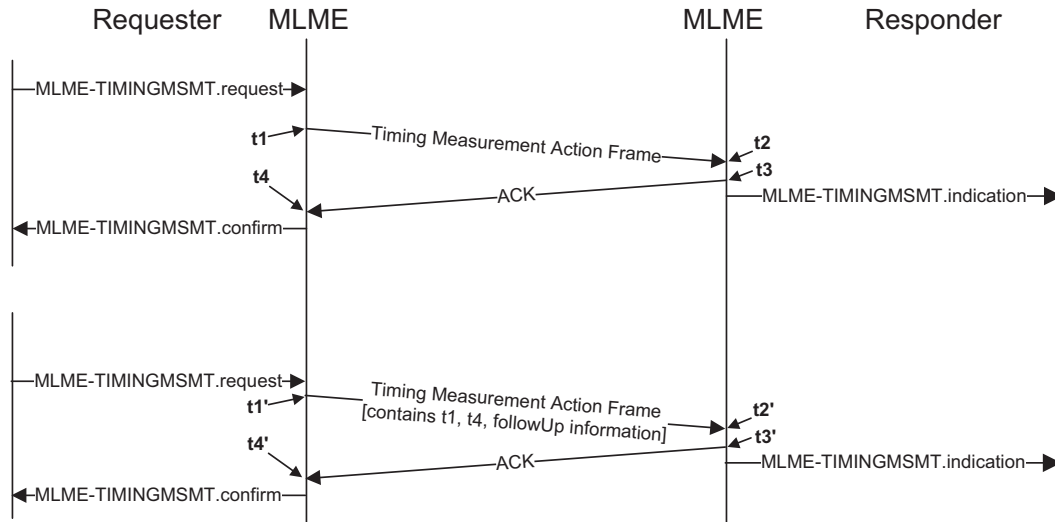
Figure 12-1—Timing measurement procedure for IEEE 802.11 links
