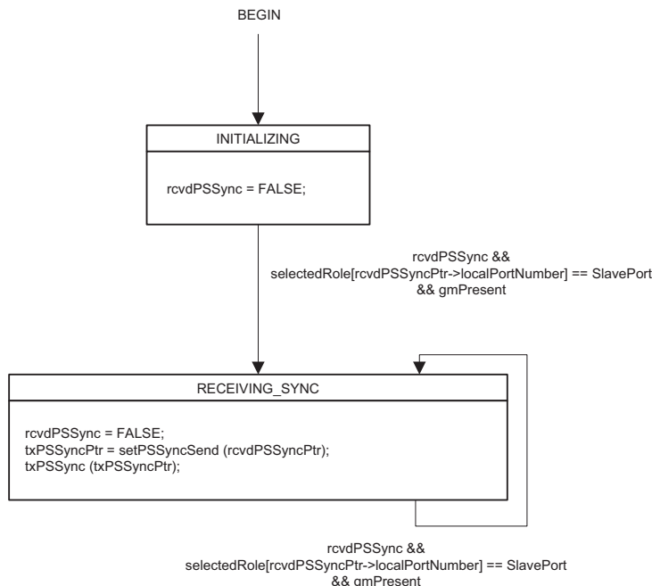
Figure 10-3—SiteSyncSync state machine
