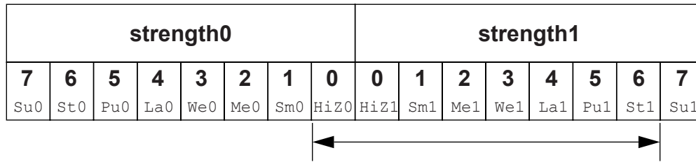
Figure 28-17—Ambiguous strength signal from a gate
