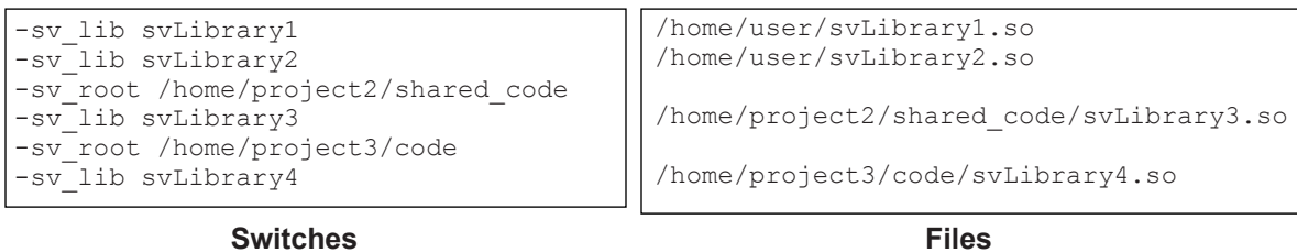
Figure J.3—Using a combination of -sv_lib and -sv_root switches
