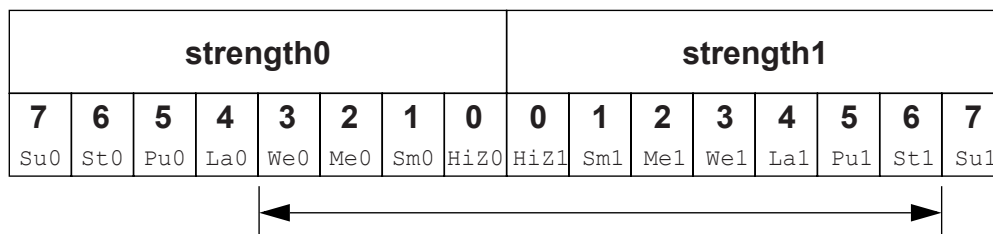
Figure 28-19—Ambiguous strength in combined gate signals
