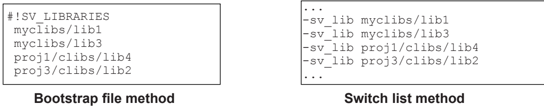
Figure J.2—Using a simple bootstrap file or a switch list
