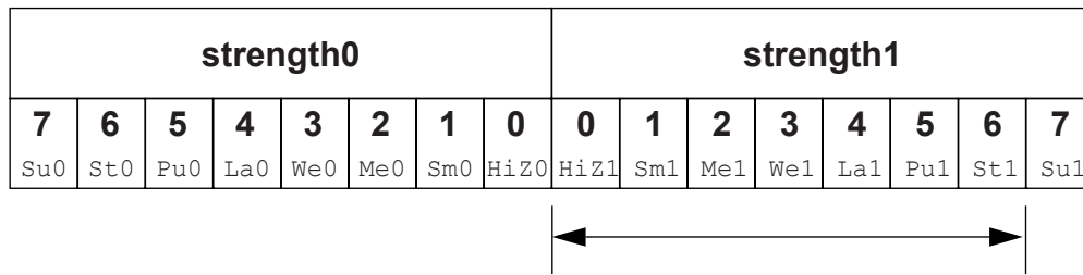
Figure 28-7—Strong H range of values
