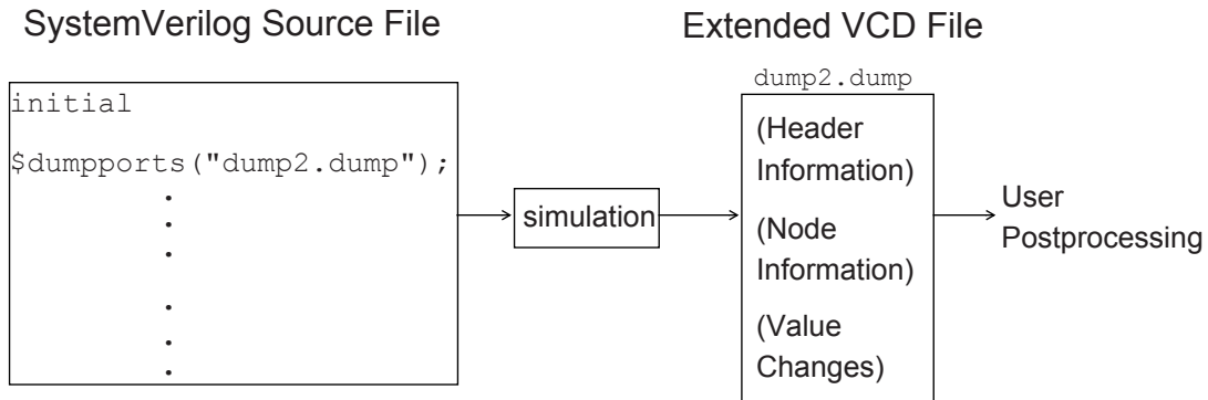
Figure 21-2—Creating the extended VCD file
