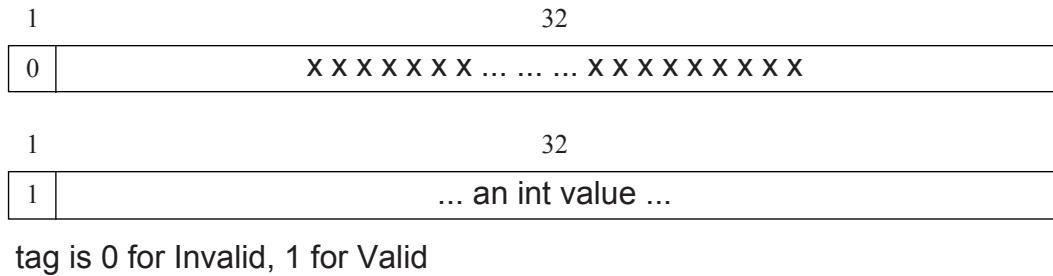
Figure 7-1—VInt type with packed qualifier
