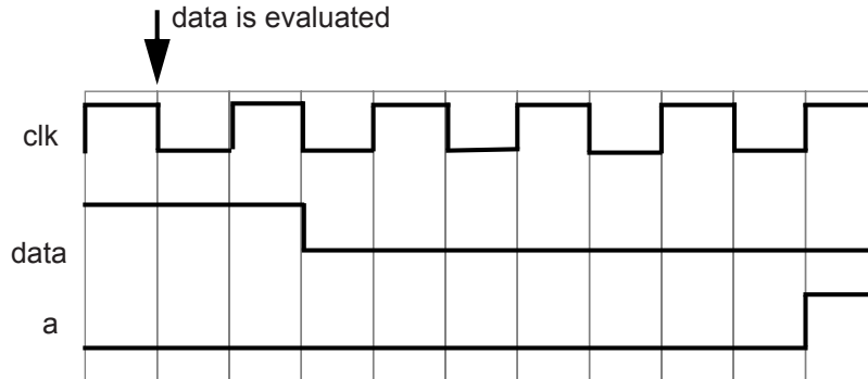
Figure 9-1—Intra-assignment repeat event control utilizing a clock edge
