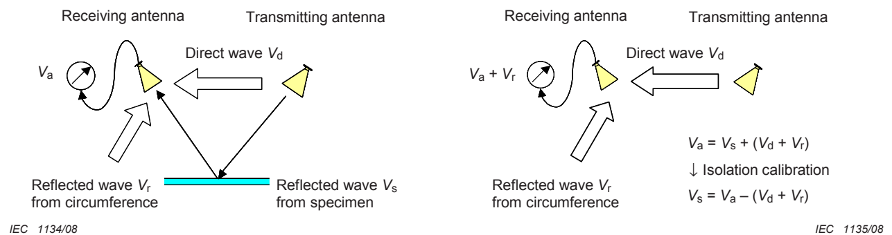
Figure F.1a – Configuration with specimen
