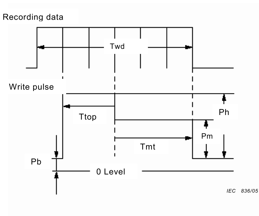
Figure A.5 – Write strategy pulse
