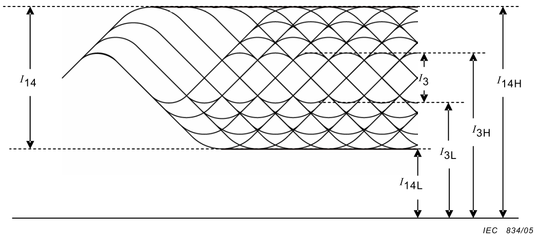
Figure A.3 – Modulation amplitude and signal asymmetry
