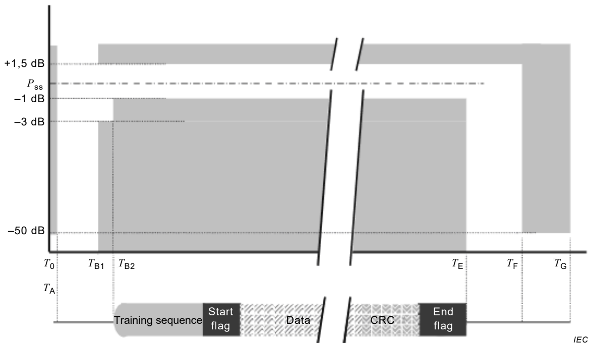
Figure 5 – Power versus time mask
