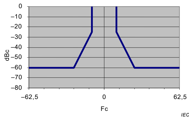
Figure 11 – Emission mask
