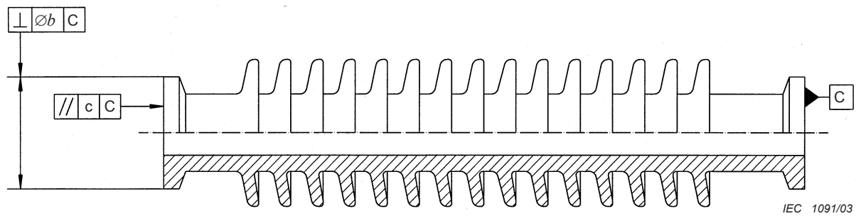
Figure A.6 – Axial run-out
