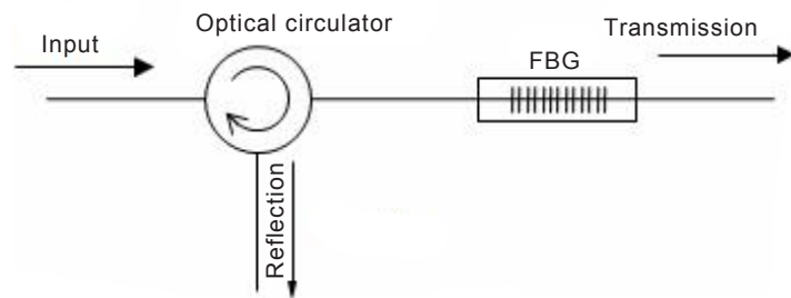
Figure B.1 – Example of application of a circulator
