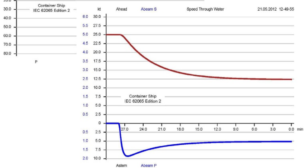
Figure I.8 – Turning circle manoeuvre – Container ship
