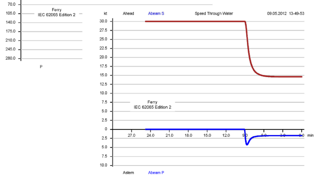
Figure I.7 – Turning circle manoeuvre – Ferry
