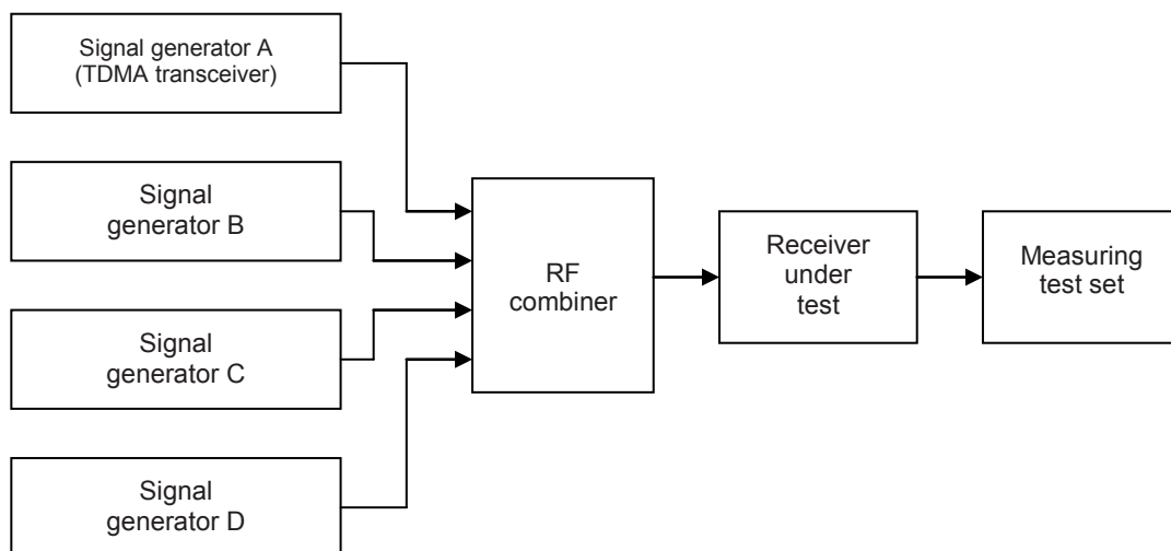
Figure 11 – Test set-up
