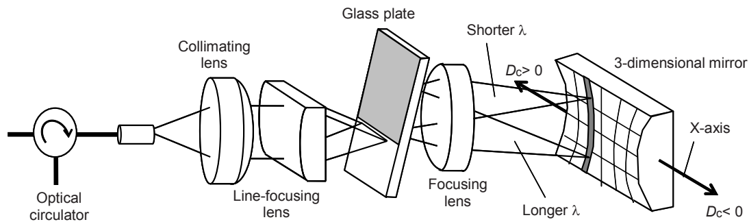
Figure C.1 – Structure of virtually imaged phased array (VIPA)
