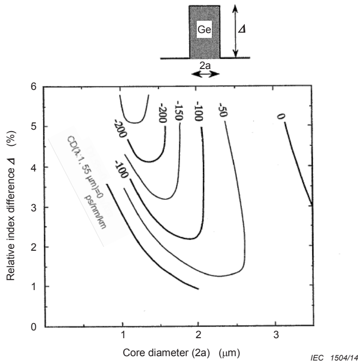
Figure A.2 – Calculated contour for different dispersion at the wavelength of 1,55 μm (CD(λ:1,55 μm)) for a step index core fibre
