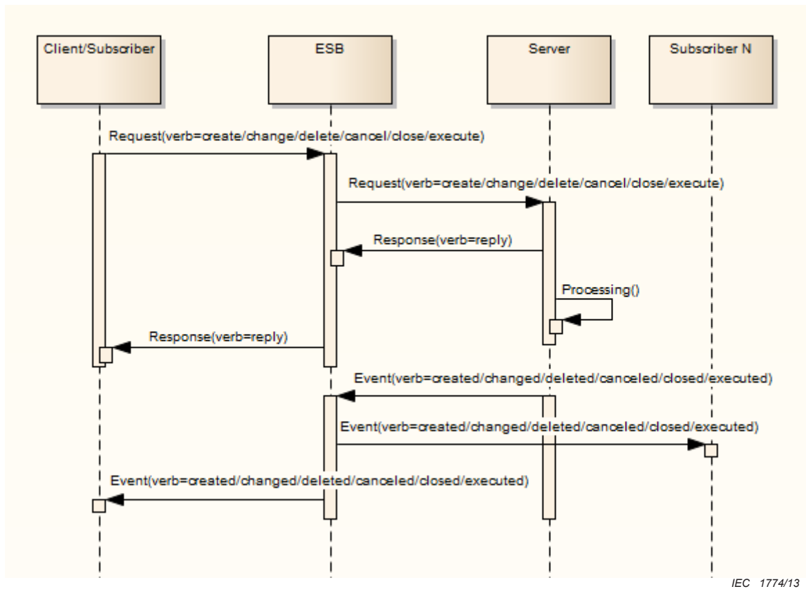
Figure 6 – Transaction Example
