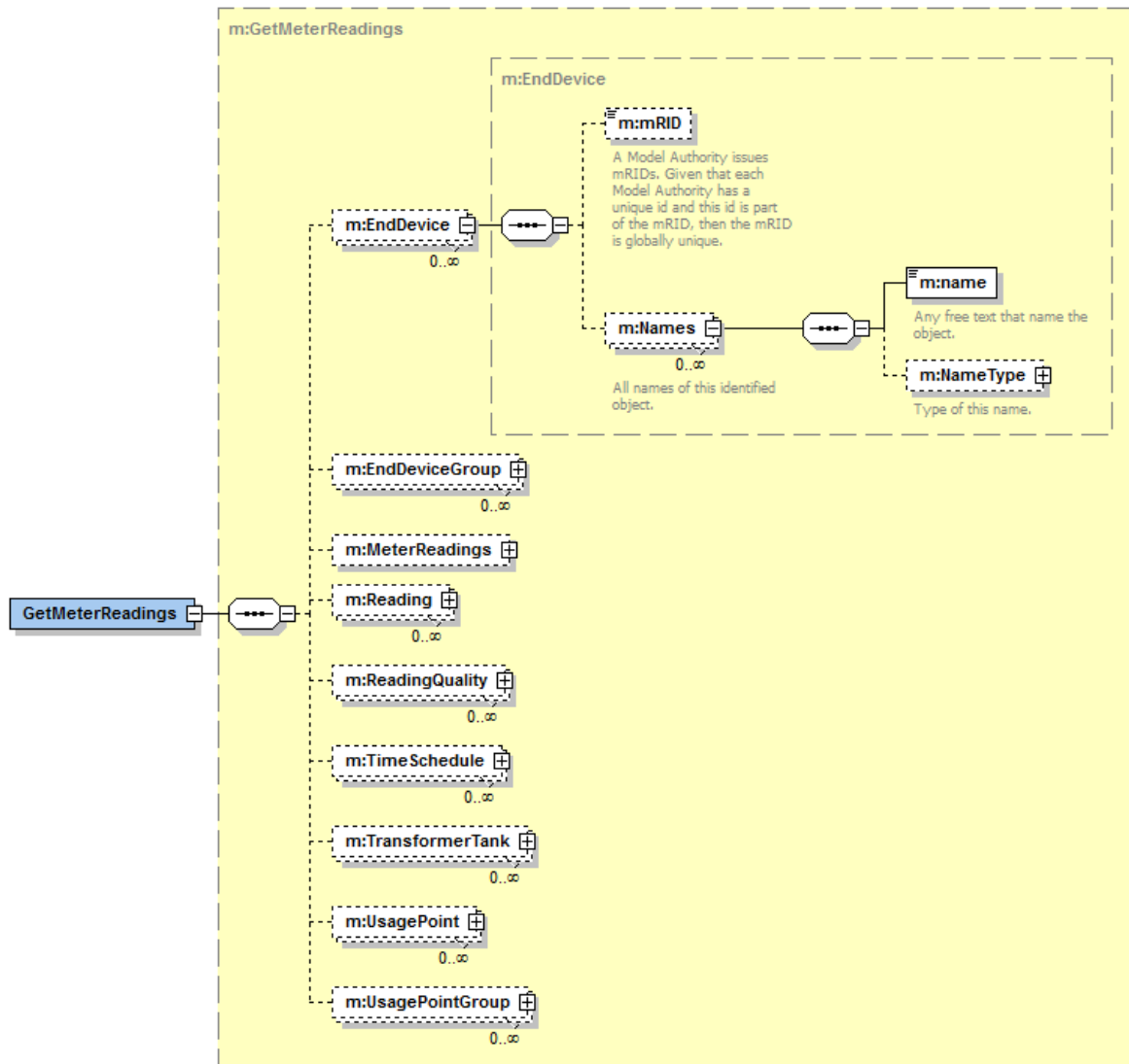
Figure 25 – Example 'Get<Noun>' profile
