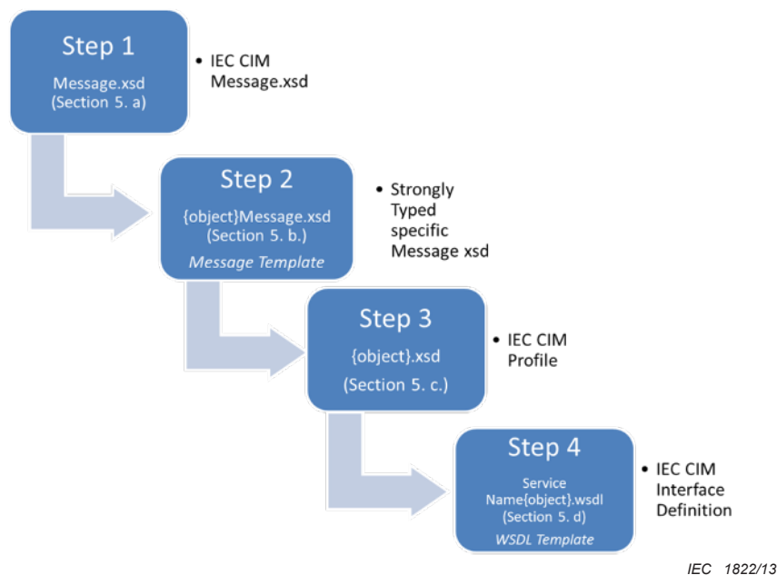
Figure C.1 – Process for WSDL Generation
