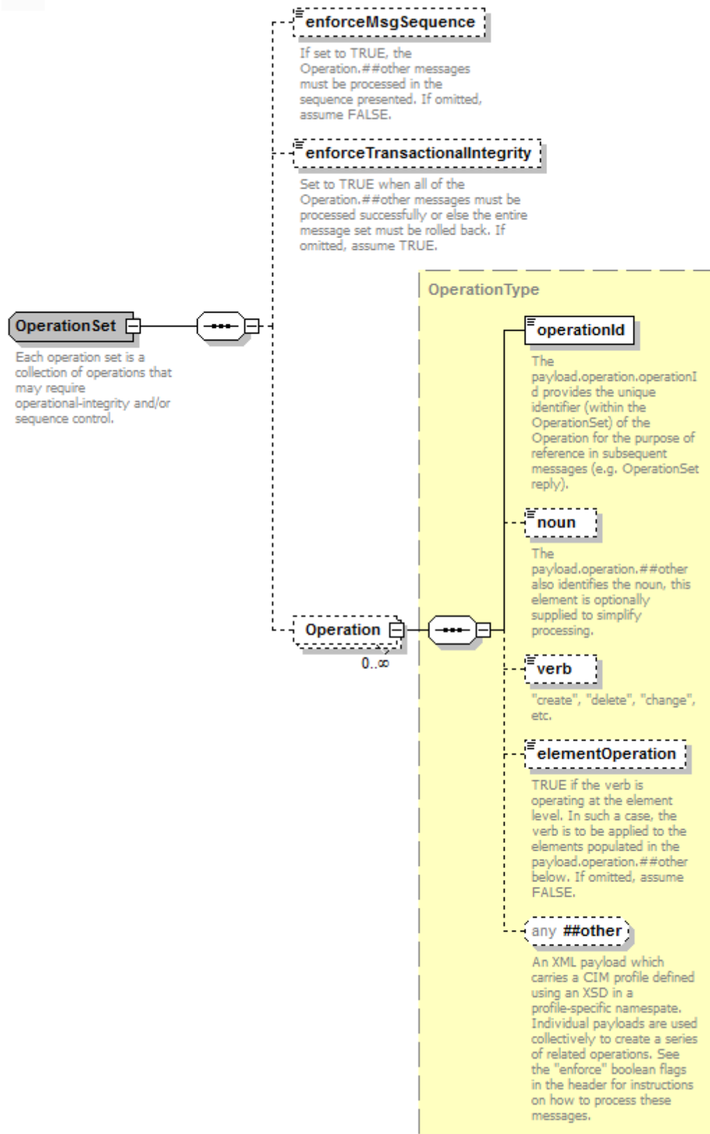
Figure 40 – OperationSet details
