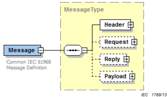
Figure 21 – Common message envelope
