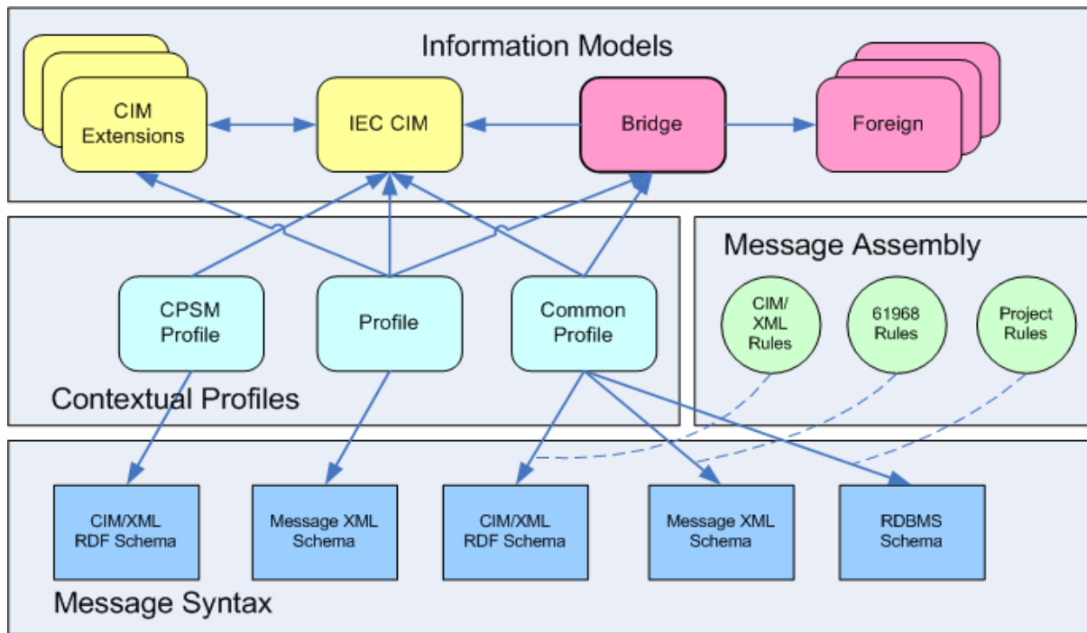
Figure 45 – Information Models, Profiles and Messages
