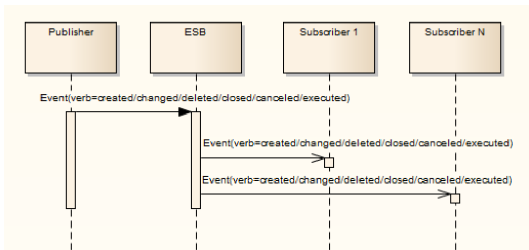
Figure 4 – Events
