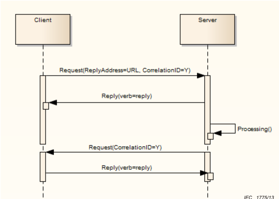
Figure 7 – Callbacks
