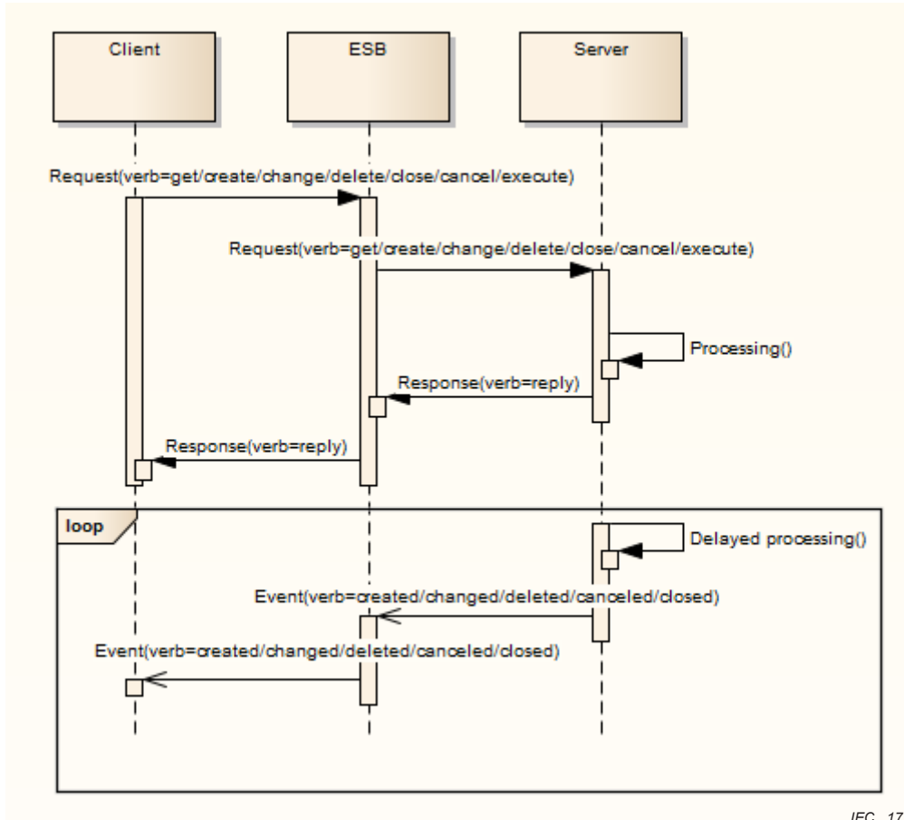
Figure 9 – Complex messaging
