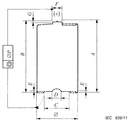
Figure 3 – Jacketed cells dimensionally interchangeable with primary cells
