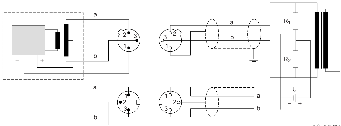
Figure 5 – Example of phantom power supply system
