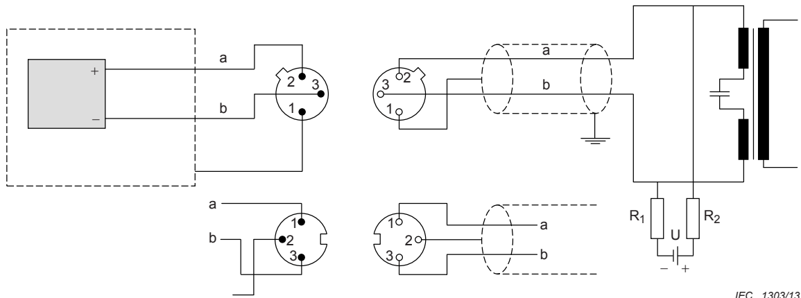
Figure 6 – Example of A-B power supply system
