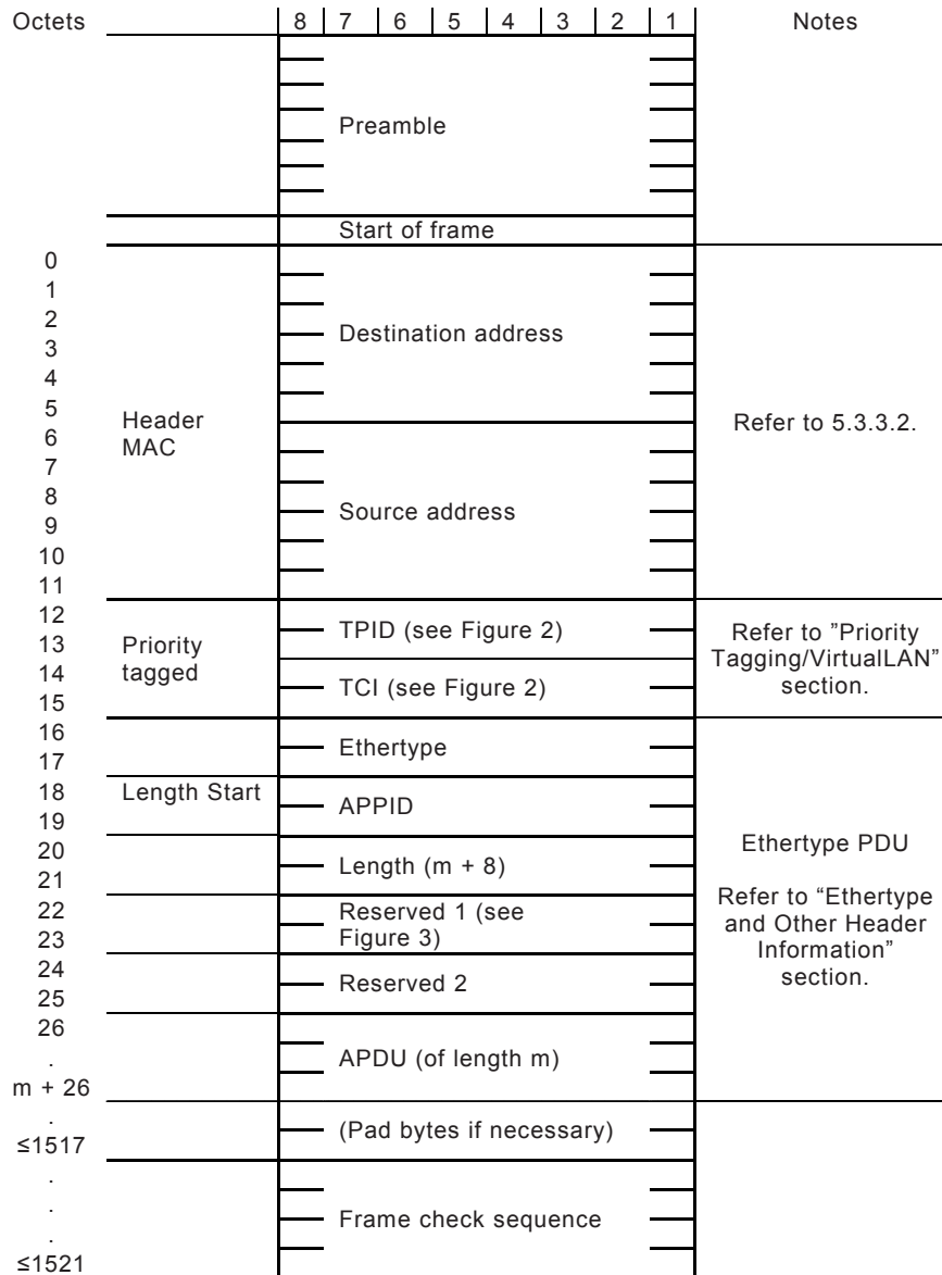
Figure A.1 – ISO/IEC 8802-3 frame format – No link redundancy
