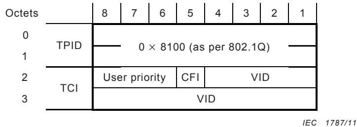
Figure 2 – Structure of the tag header
