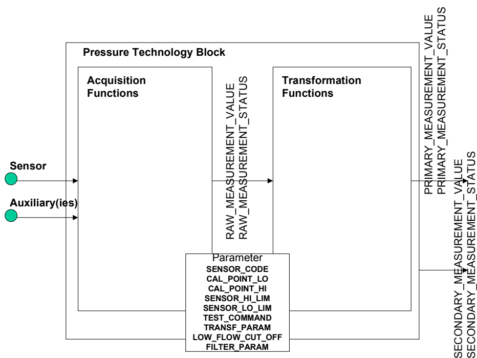
Figure 19 – Pressure Technology Block
