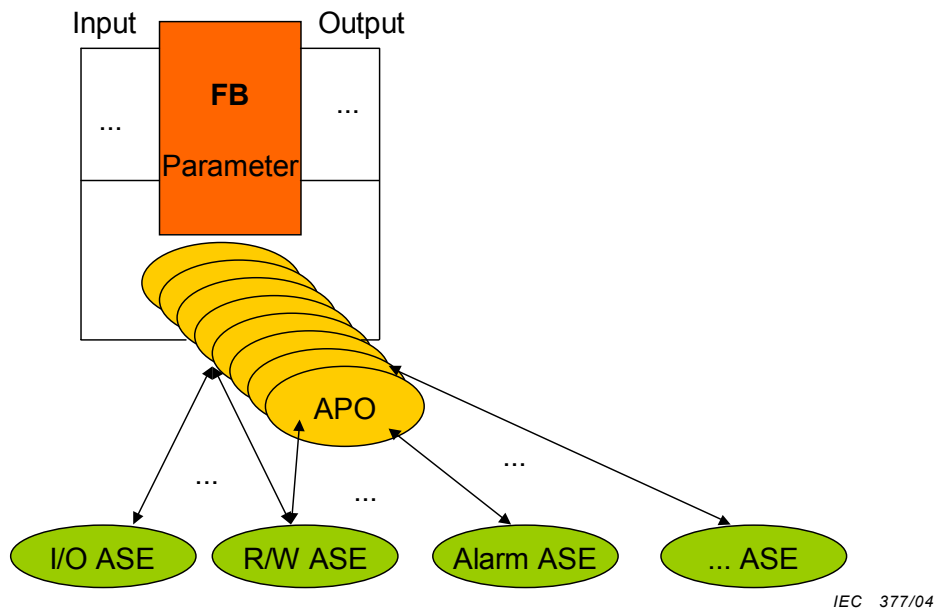
Figure 25 – Mapping of IEC 61804 FBs to APOs
