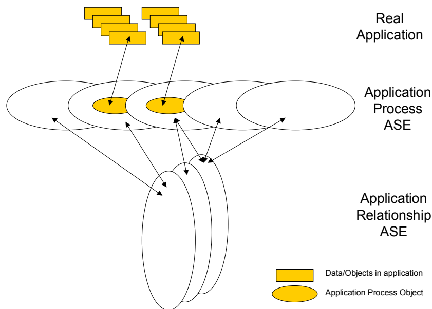
Figure 23 – Application structure of ISO OSI Reference Model
