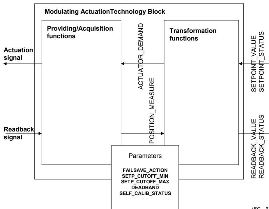
Figure 20 – Modulating actuation technology block
