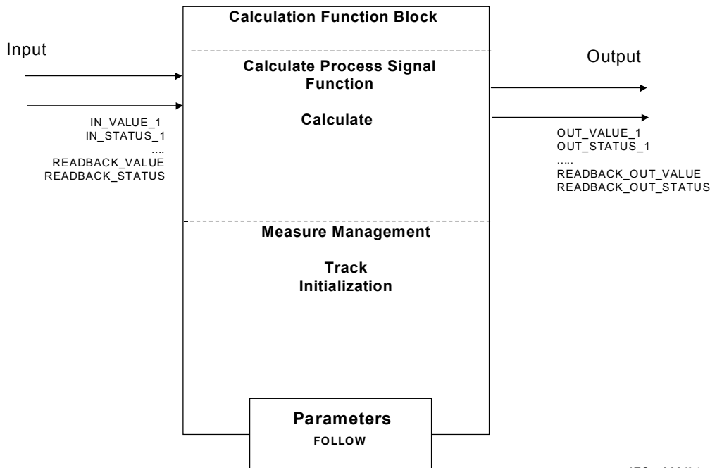
Figure 16 – Calculation FB
