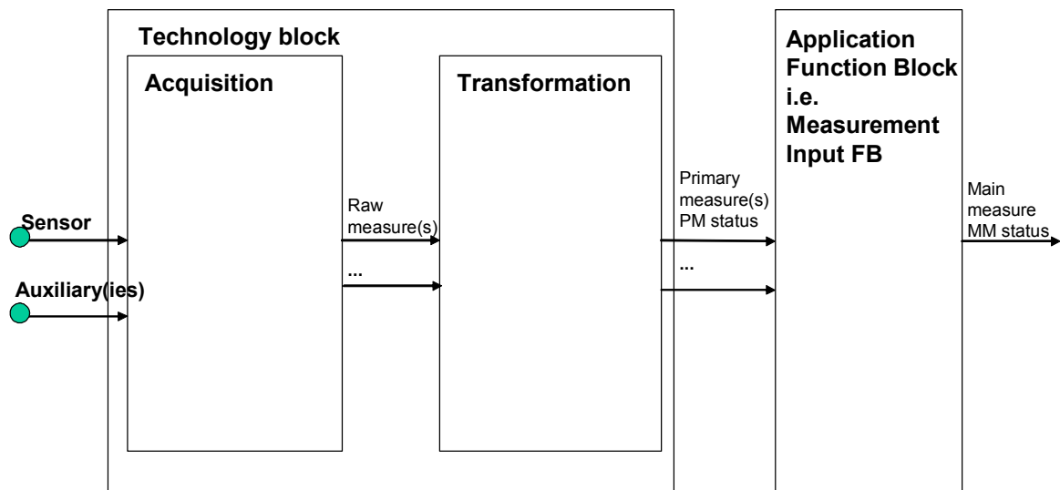
Figure 9 – Measurement process signal flow
