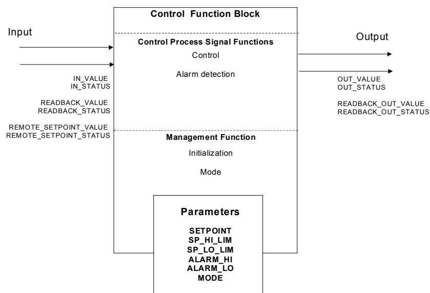
Figure 17 – Control FB
