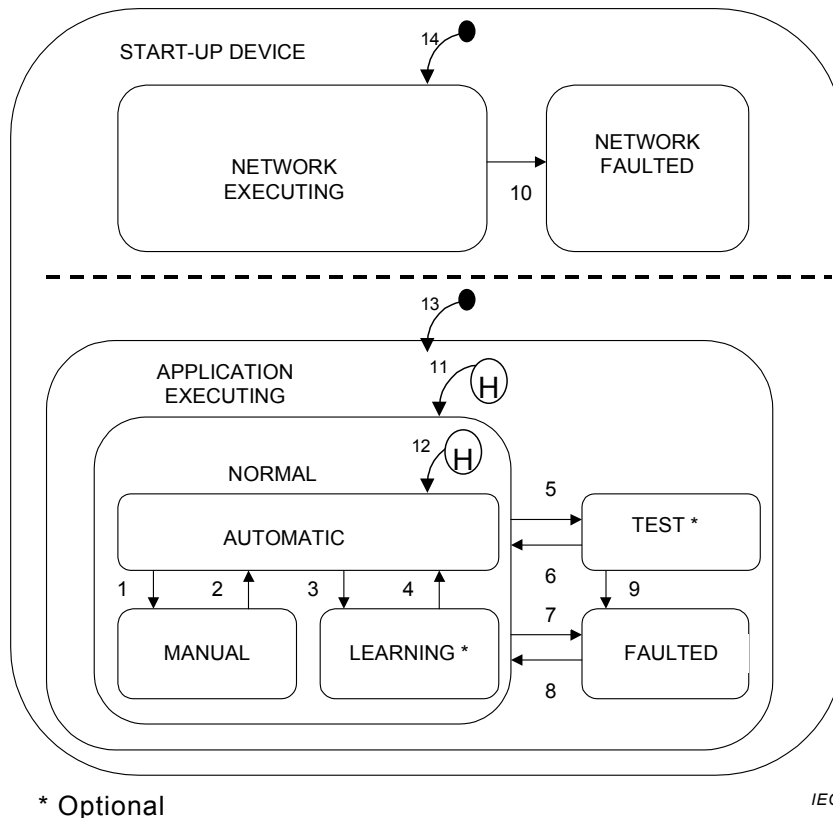
Figure 22 – Harel state chart
