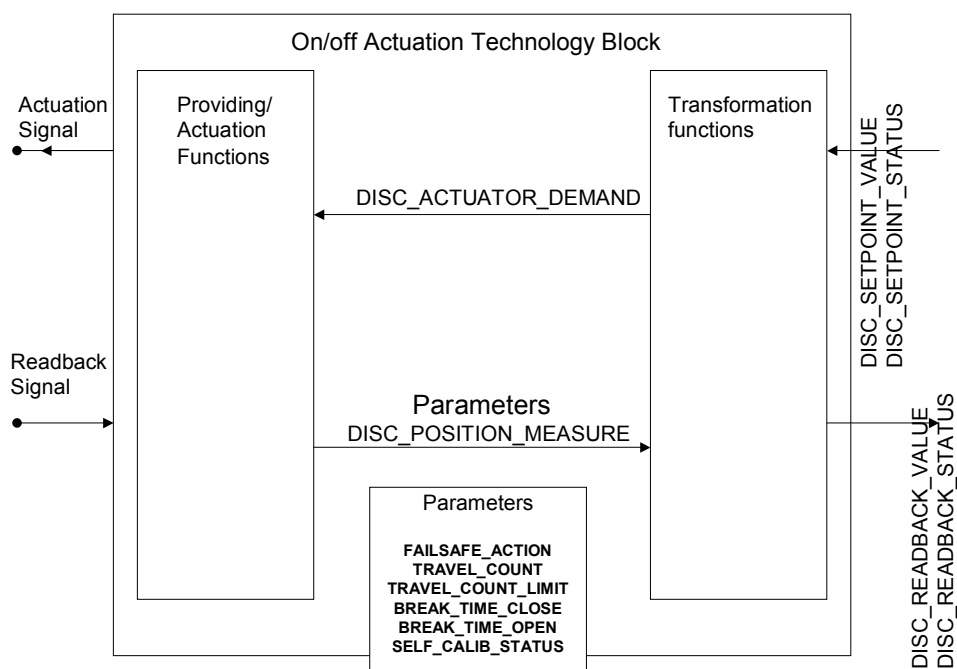
Figure 21 – On/Off Actuation Technology Block
