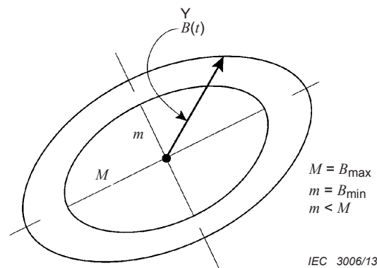
Figure C.1a – Quantities for elliptical polarization, m < M
