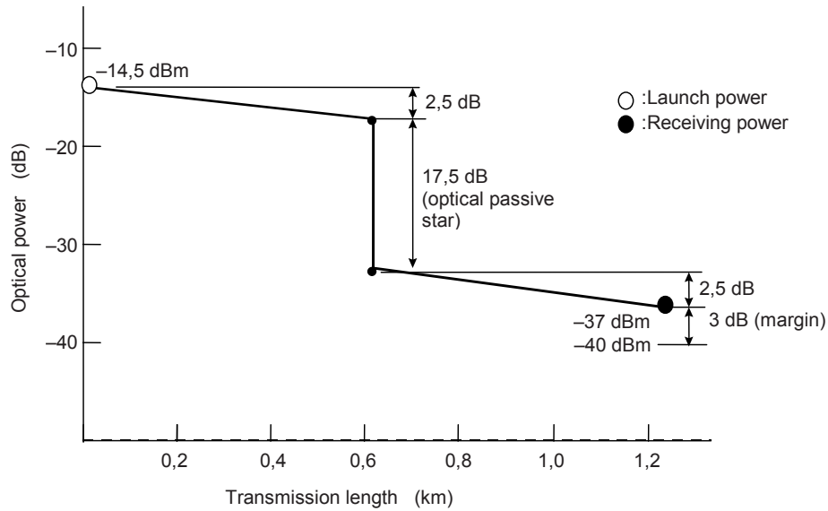
Figure 2 – Example optical power budget for a 100/140 μm fiber system with a 16/16 optical passive star coupler
